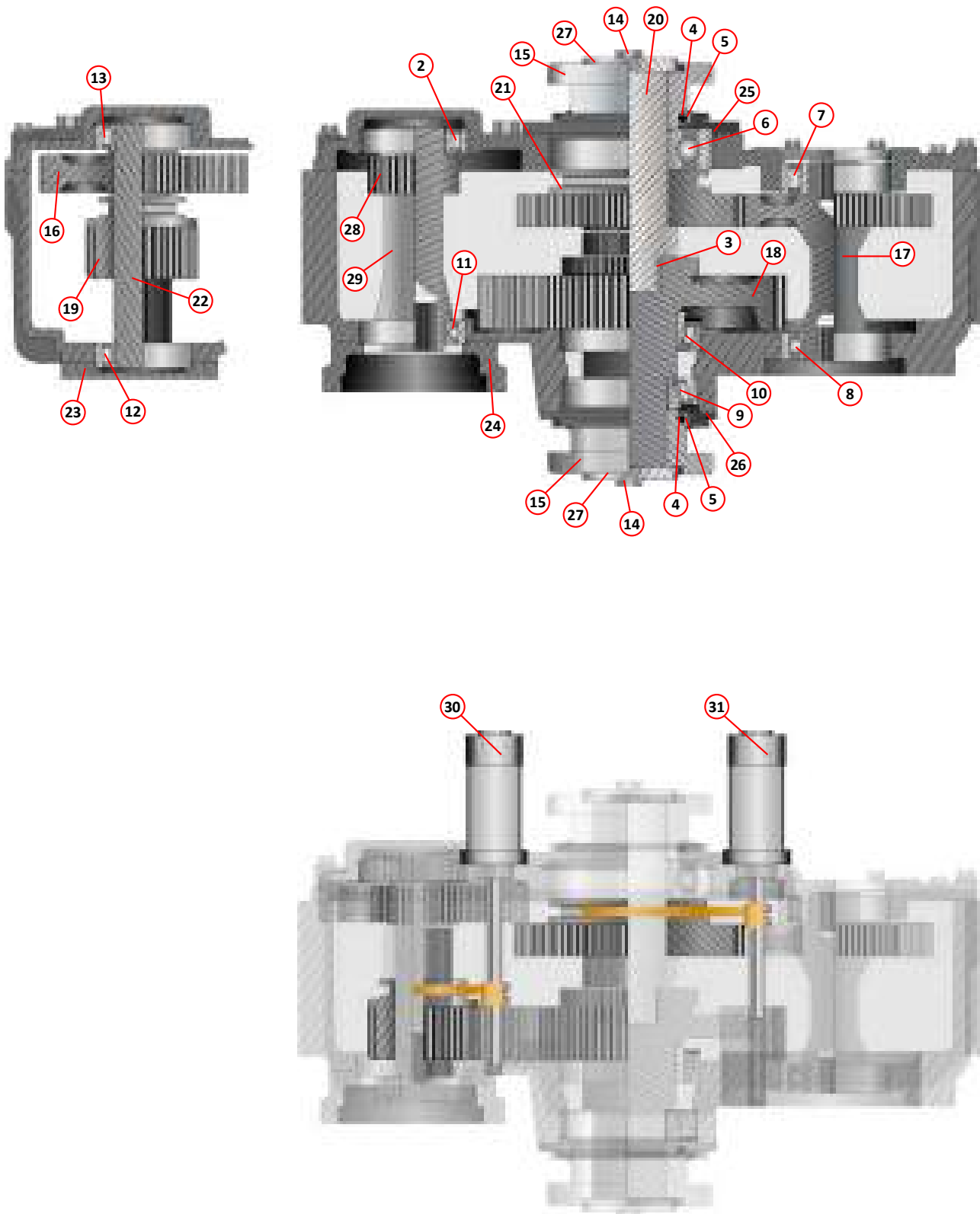
Rögelberg Gearbox HP Type Ratio Build Configurations
