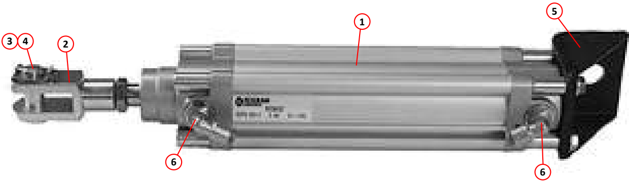
Wide Sweep Raise / Lower Cylinder
