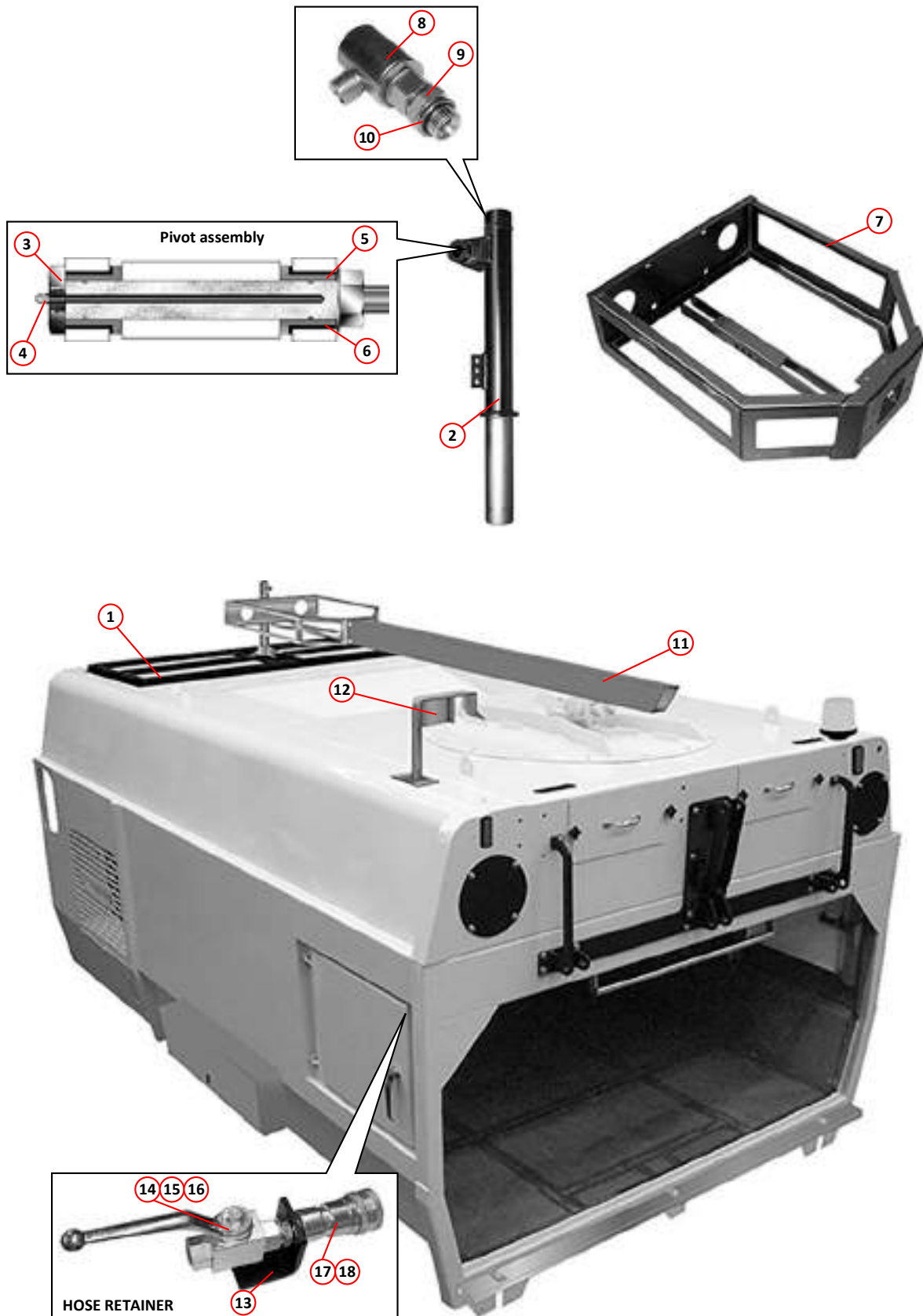
Water Boom Assembly - Merlin and Magnum
