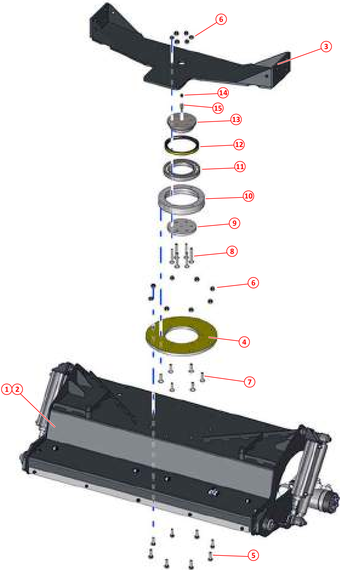
Figure 48: Slew bearing arrangement, central brush (wide sweep)
