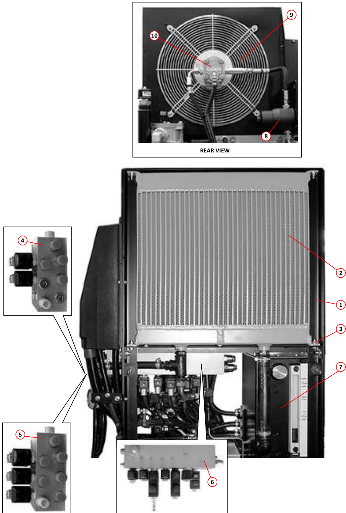
Gantry General Arrangement
