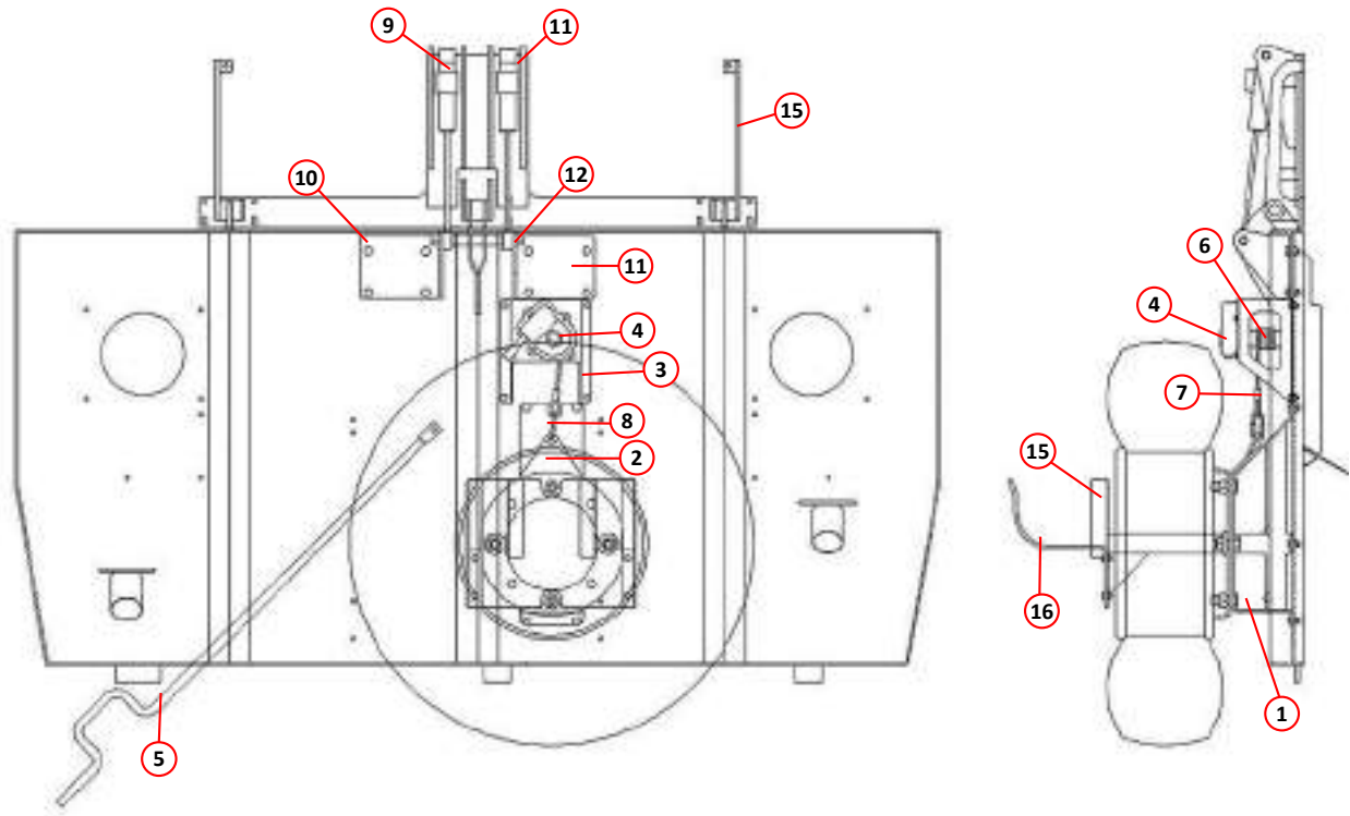
Spare Wheel Carrier - Magnum
