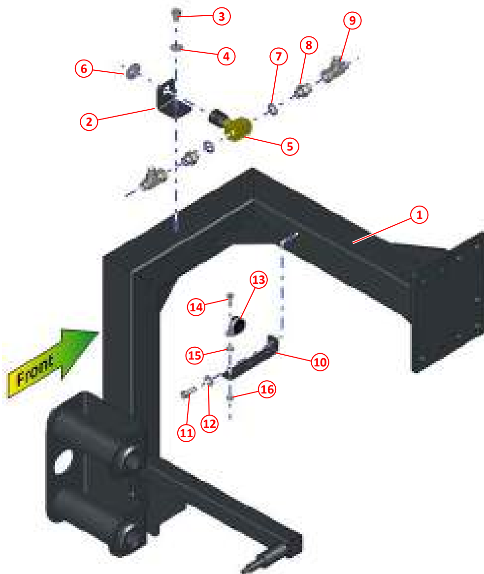
Figure 96: Brush speed control, auxiliary brush, right hand
