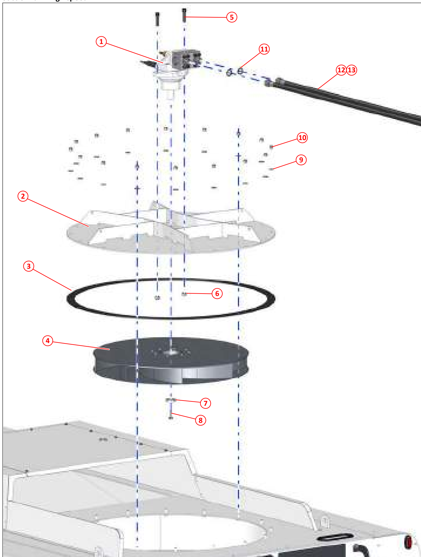
Figure 100: Suction fan - high speed
