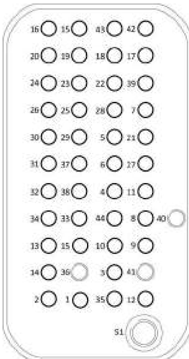
Bulkhead Connectors - Pneumatic Control Box
