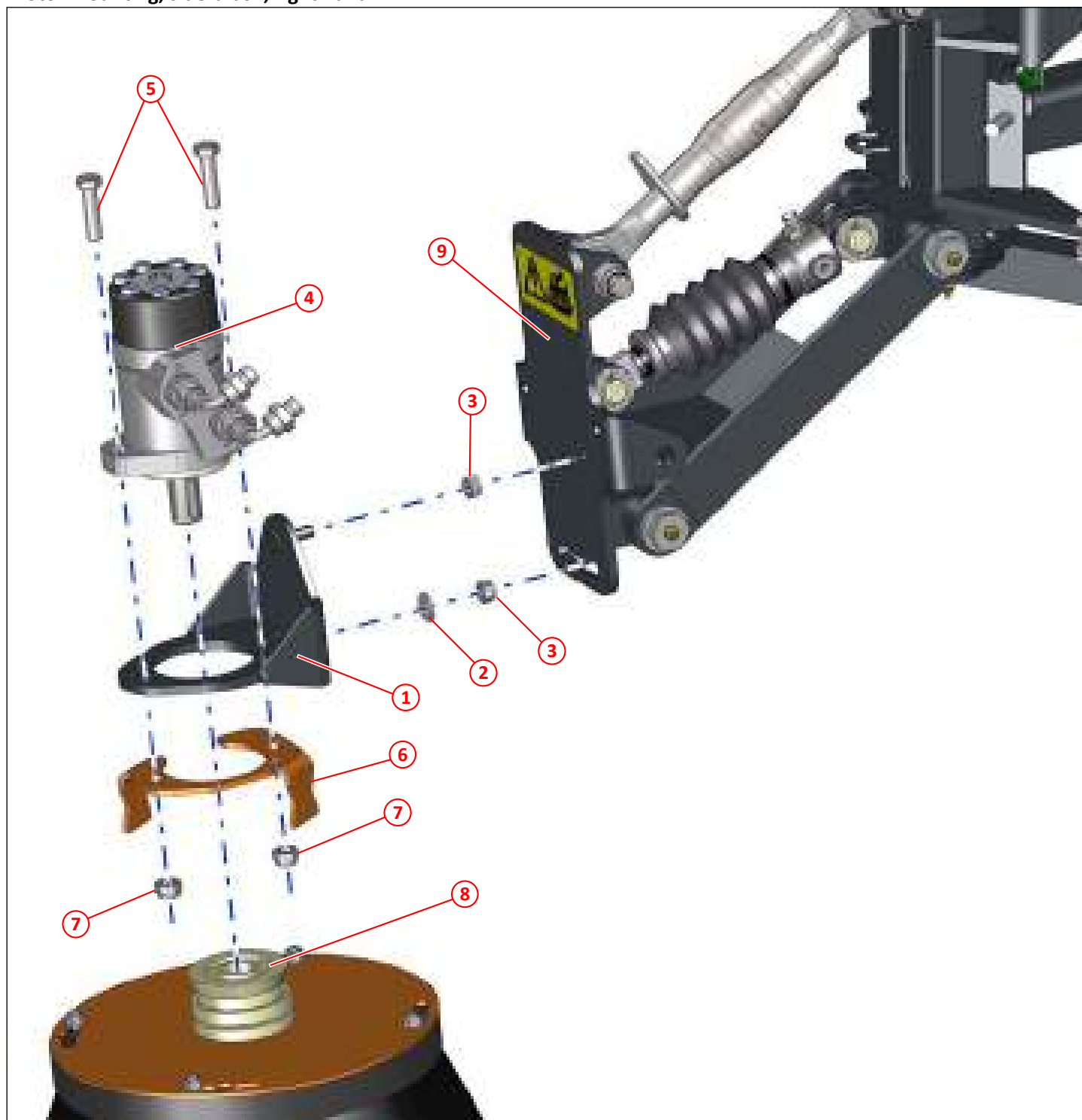
Figure 37: Motor mounting, side brush, right hand
