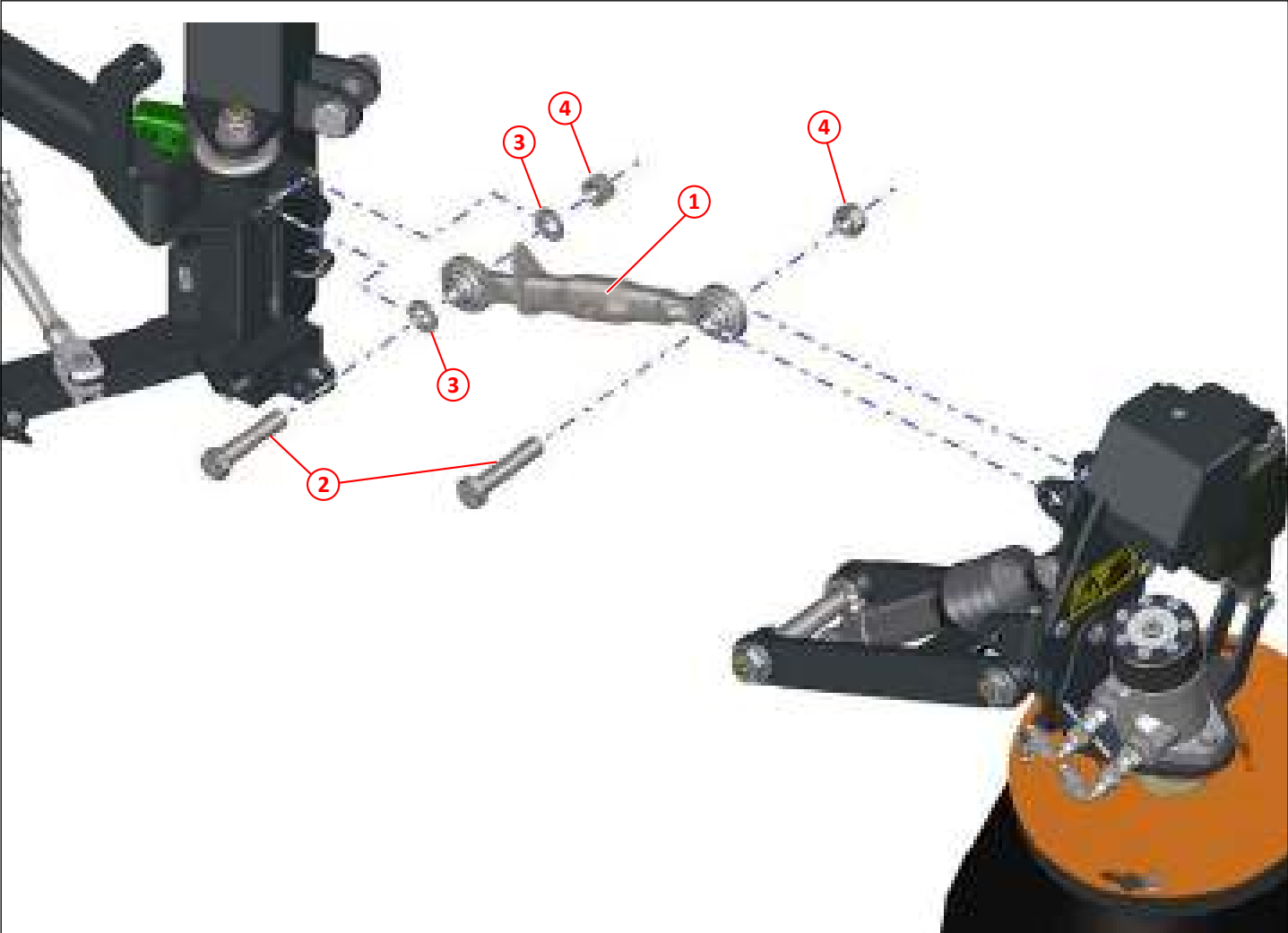
Figure 14: Top link, side brush, left hand
