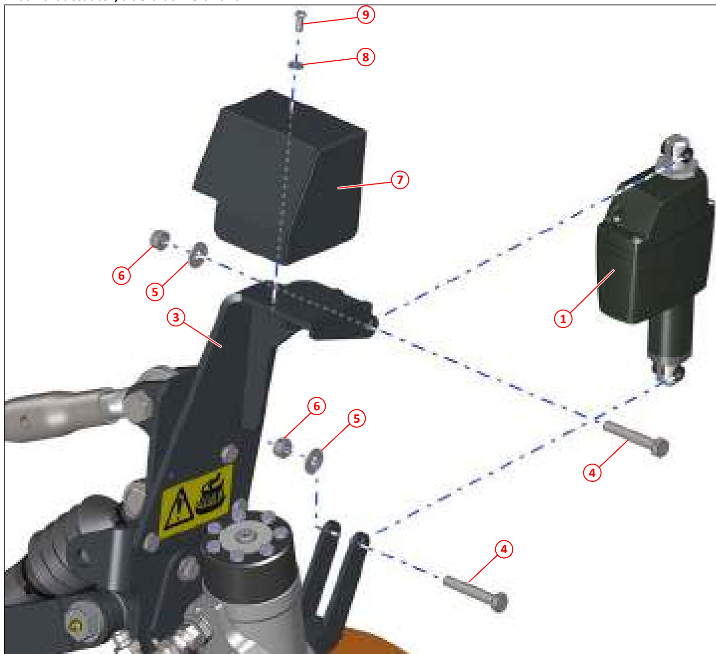
Figure 22: Brush tilt actuator, side brush left hand
