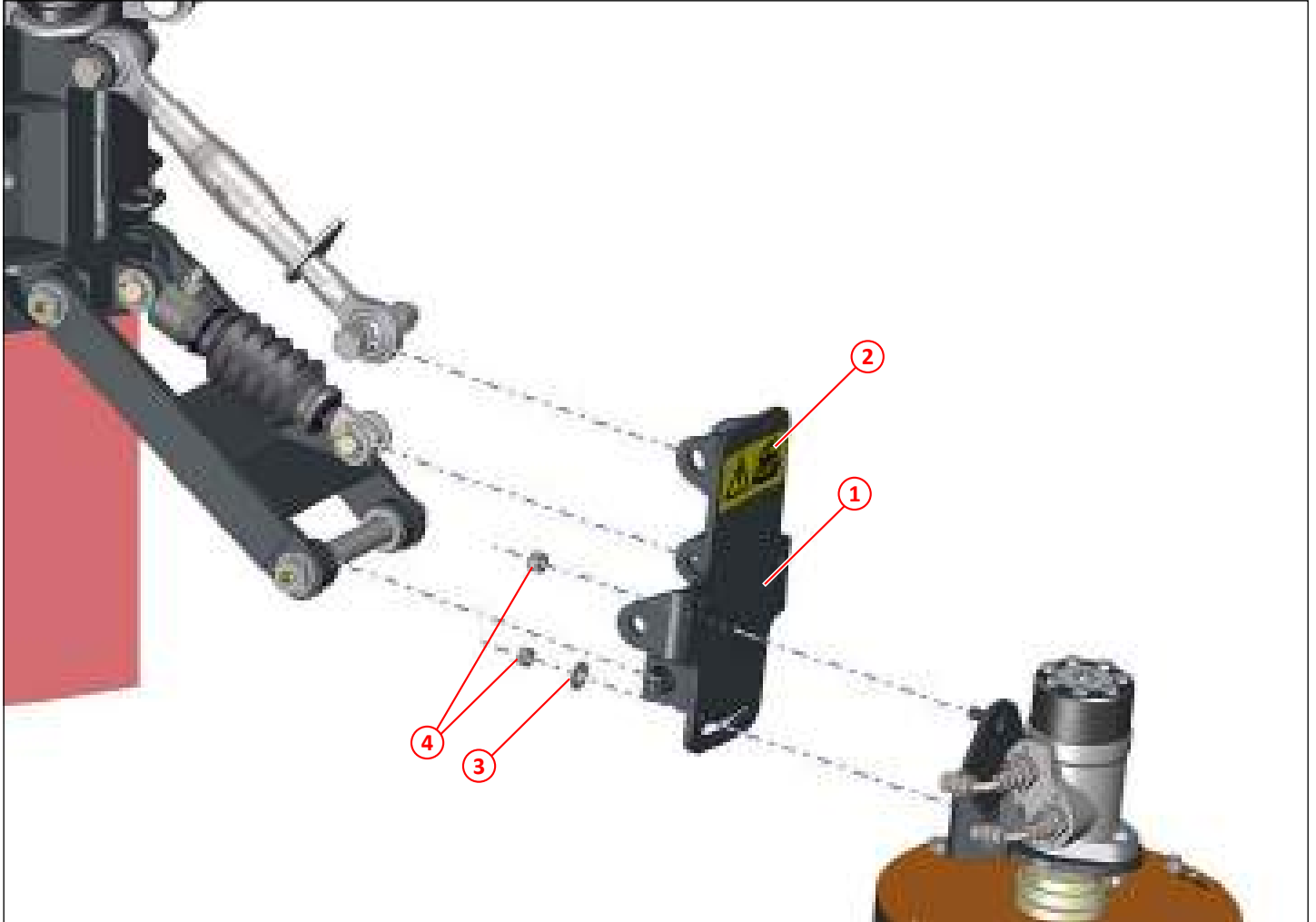
Figure 15: Swivel plate, side brush, left hand
