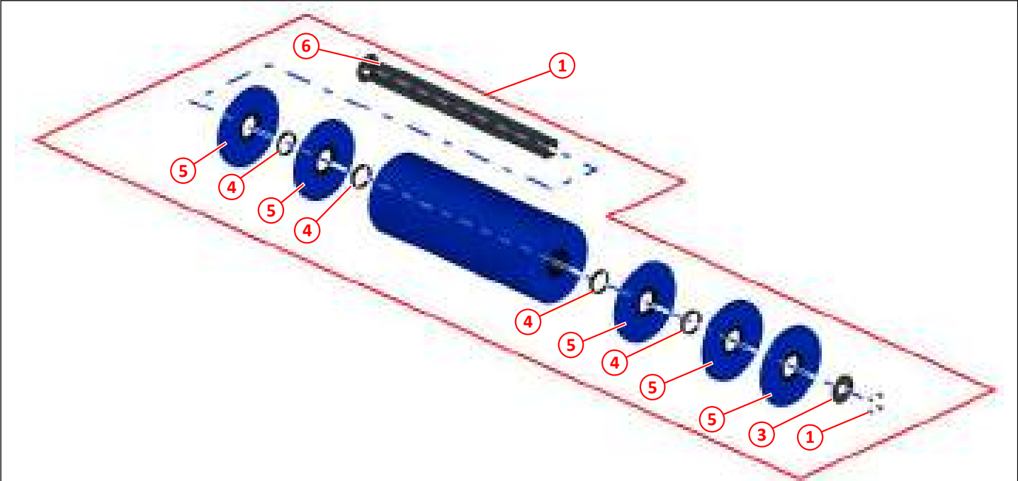
Figure 63: Brush assembly, central brush (wide sweep), standard+200mm, 400mm dia x 1235mm long
