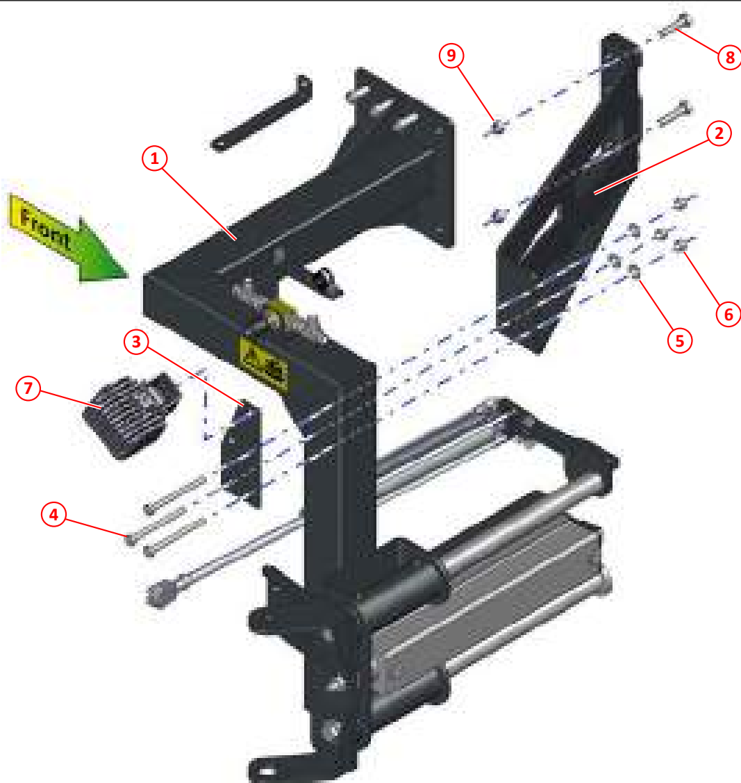
Figure 91: Support bracket and work light, auxiliary brush, right hand
