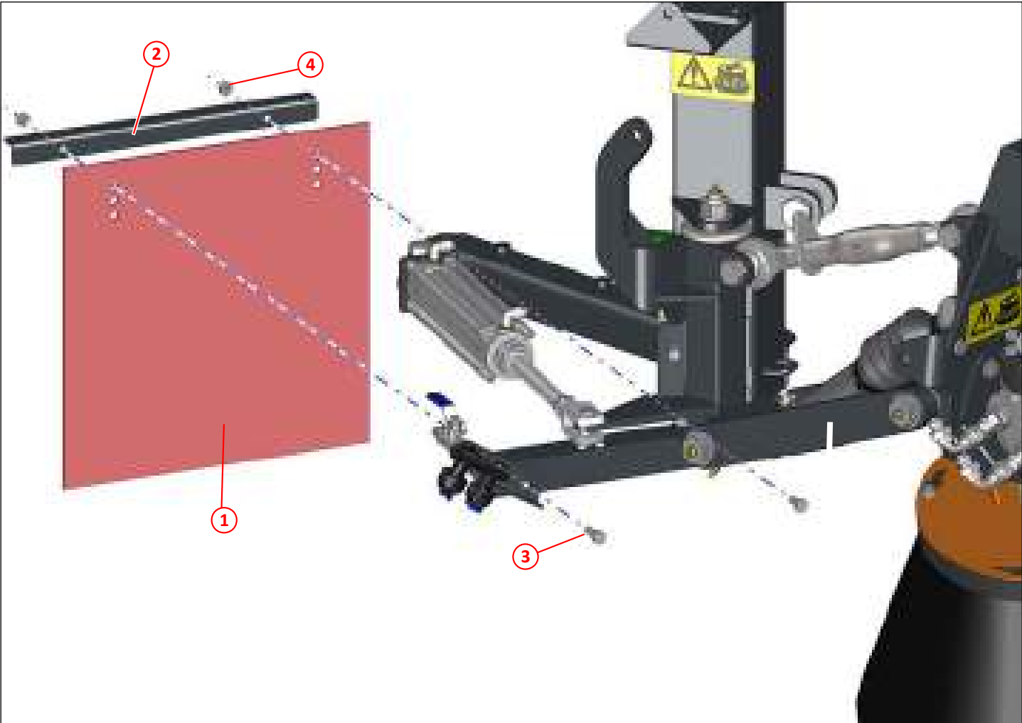
Figure 10: Skirt, side brush, left hand
