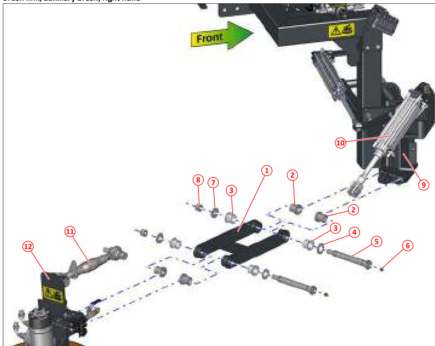
Figure 85: Brush link, auxiliary brush, right hand
