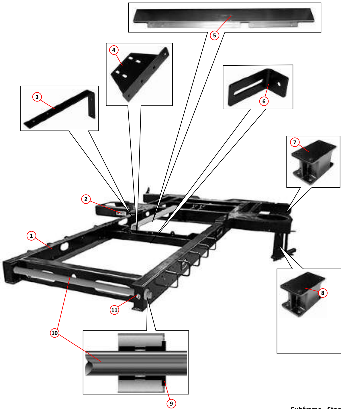
Subframe - Standard Parts
