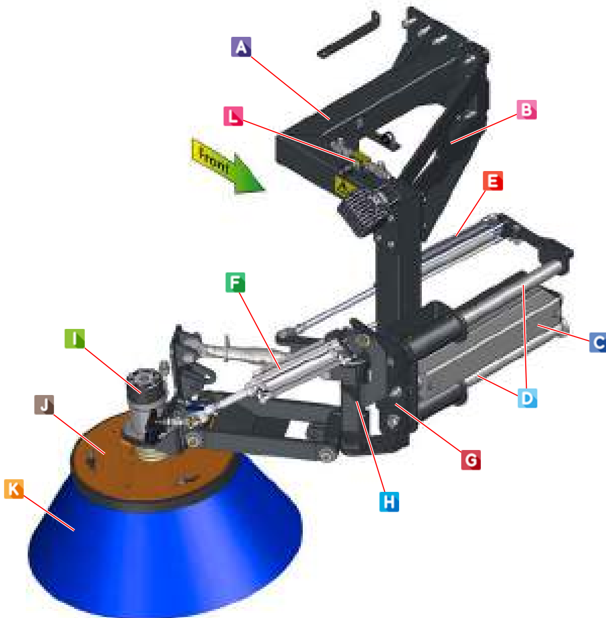
Figure 82: Auxiliary brush, right hand, general arrangement
