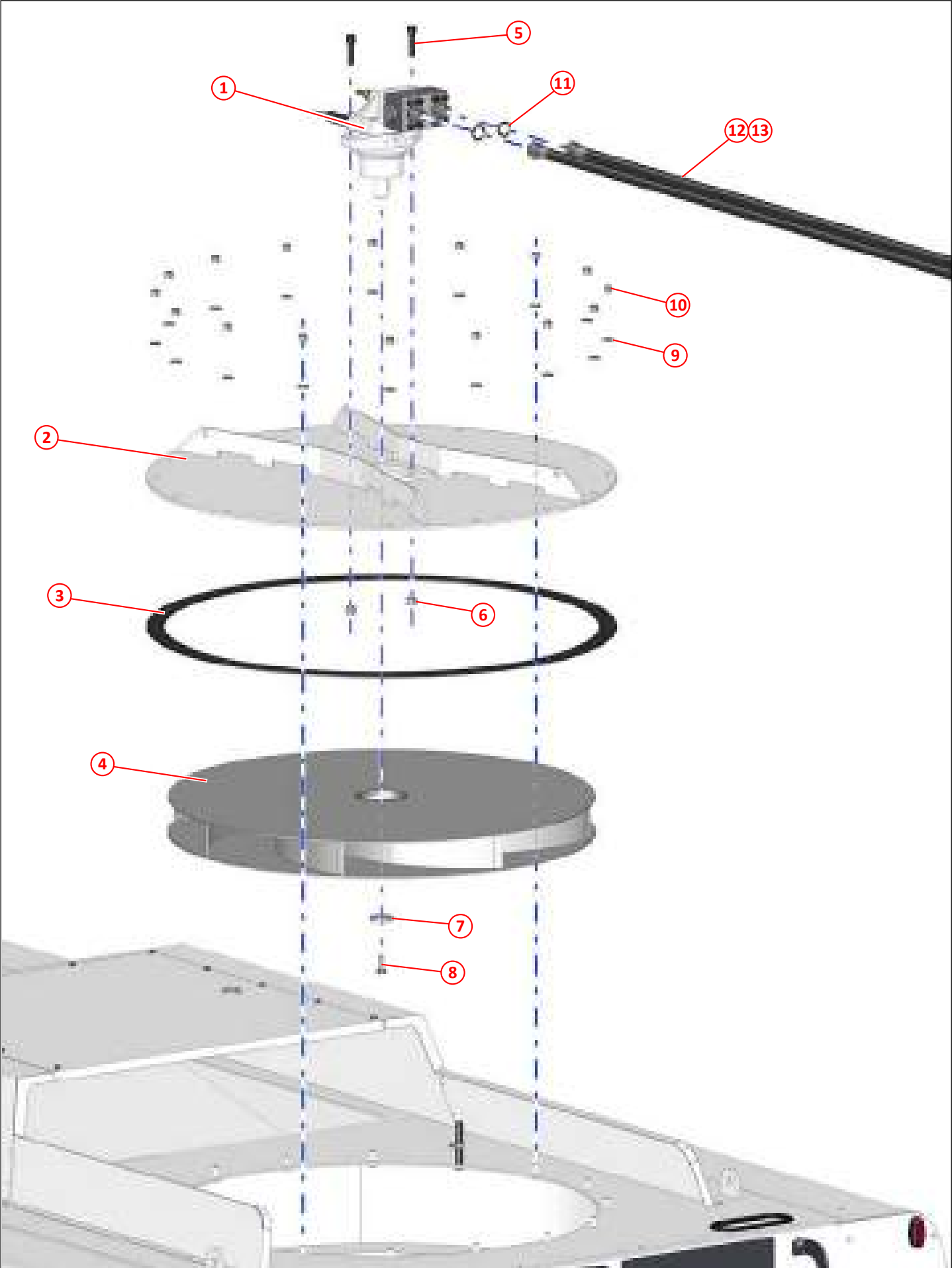
Figure 99: Suction fan - standard speed
