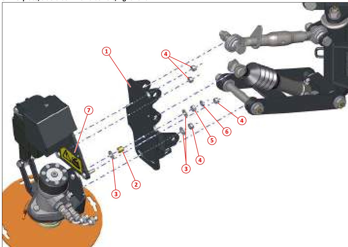
Figure 36: Swivel plate, side brush with brush tilt, right hand
