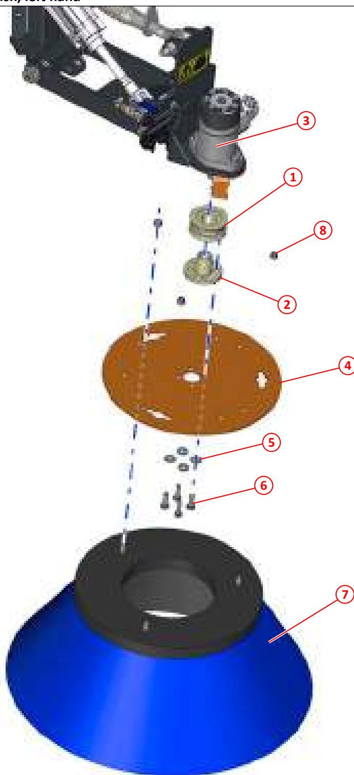
Figure 72: Brush and brush hub, auxiliary brush, left hand
