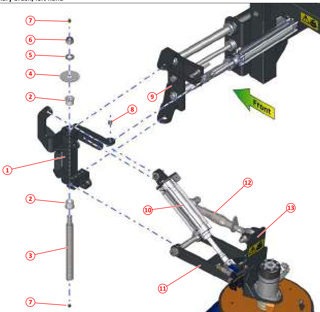
Figure 66: King post, auxiliary brush, left hand
