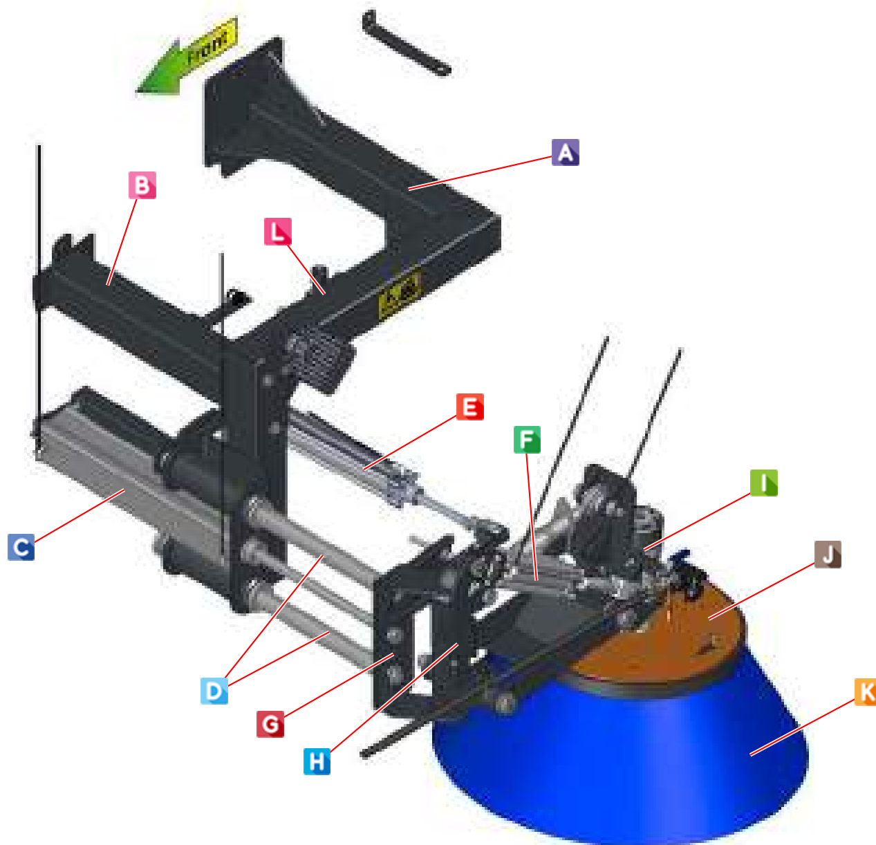
Figure 65: Auxiliary brush, left hand, general arrangement
