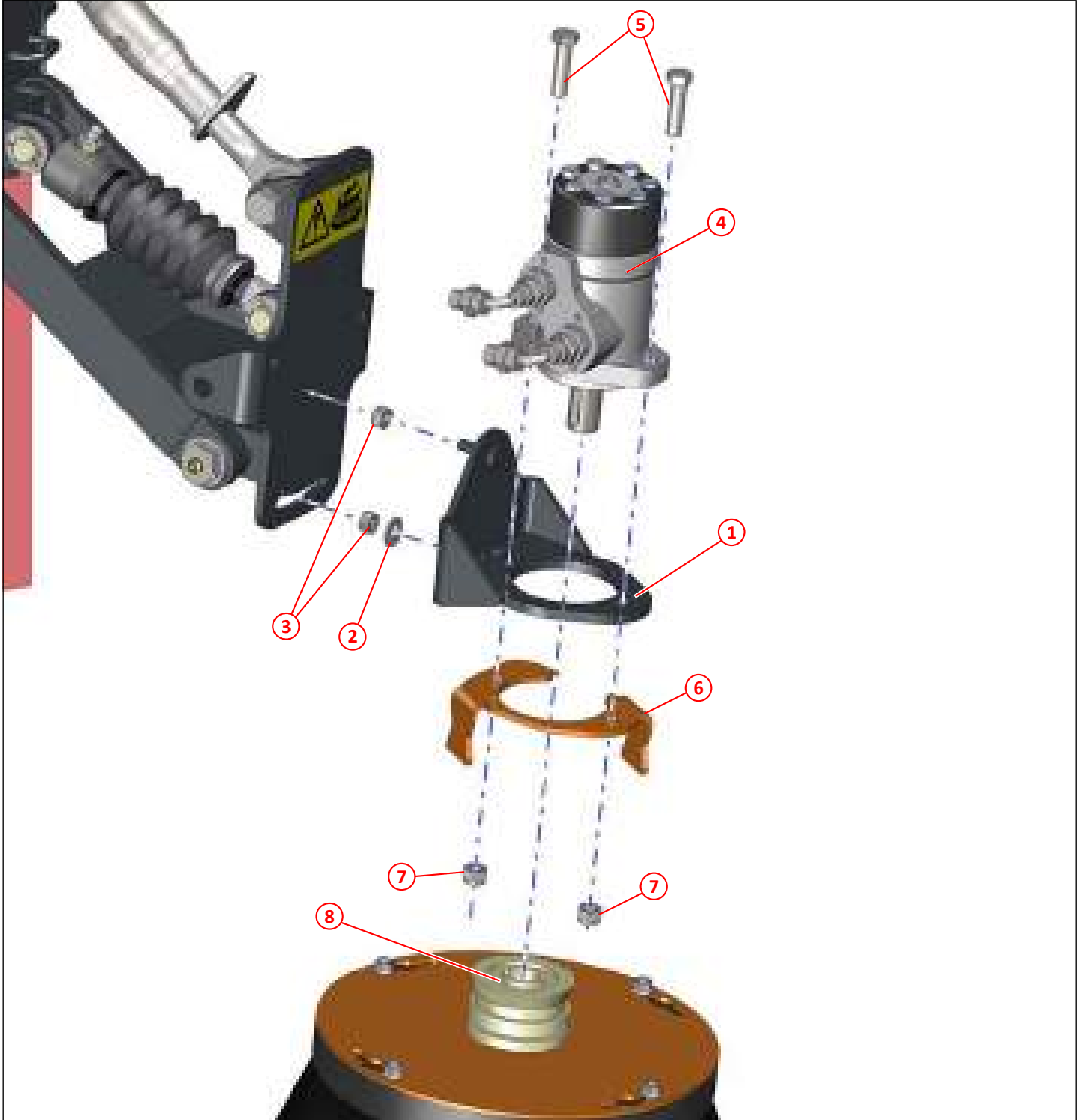
Figure 17: Motor mounting, side brush, left hand
