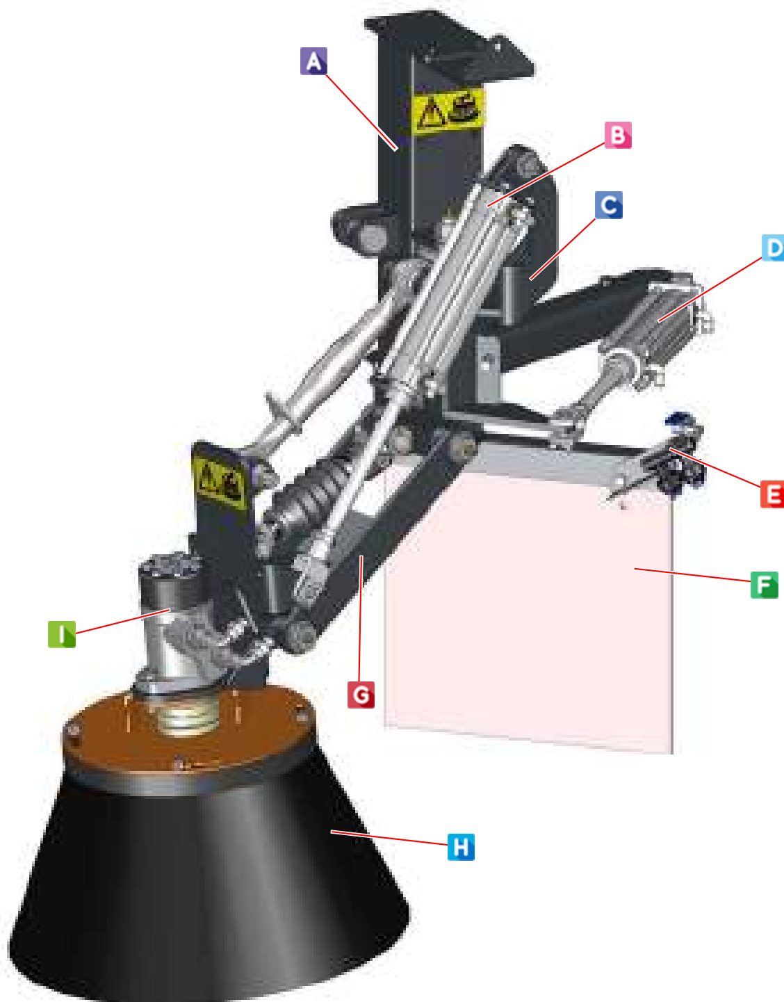
Figure 23: Side brush arrangement, right hand, without brush tilt
