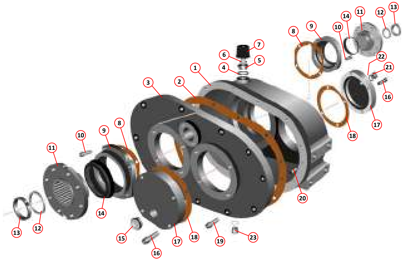
Scarab Reduction Gearbox External Parts
