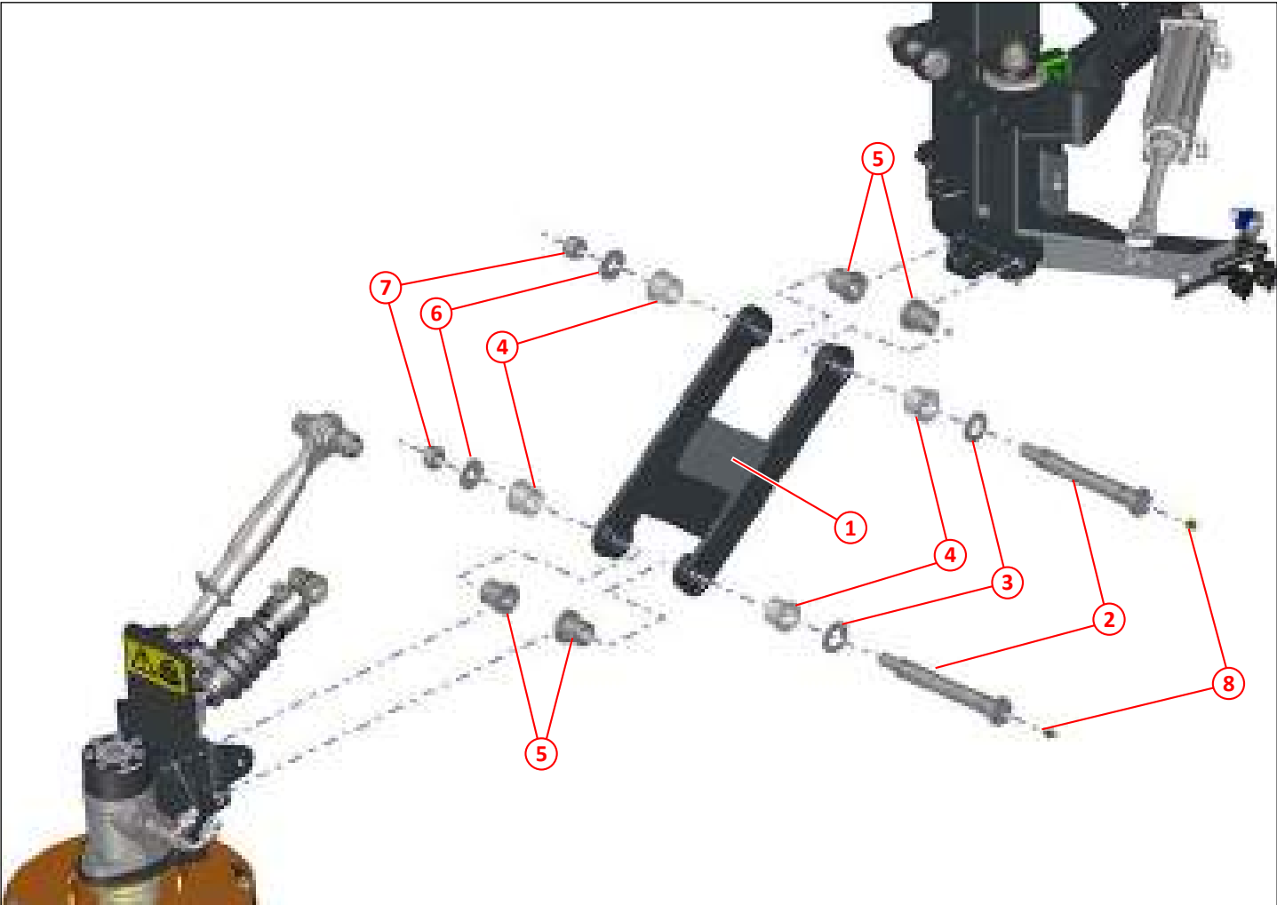
Figure 32: Brush link, right hand
