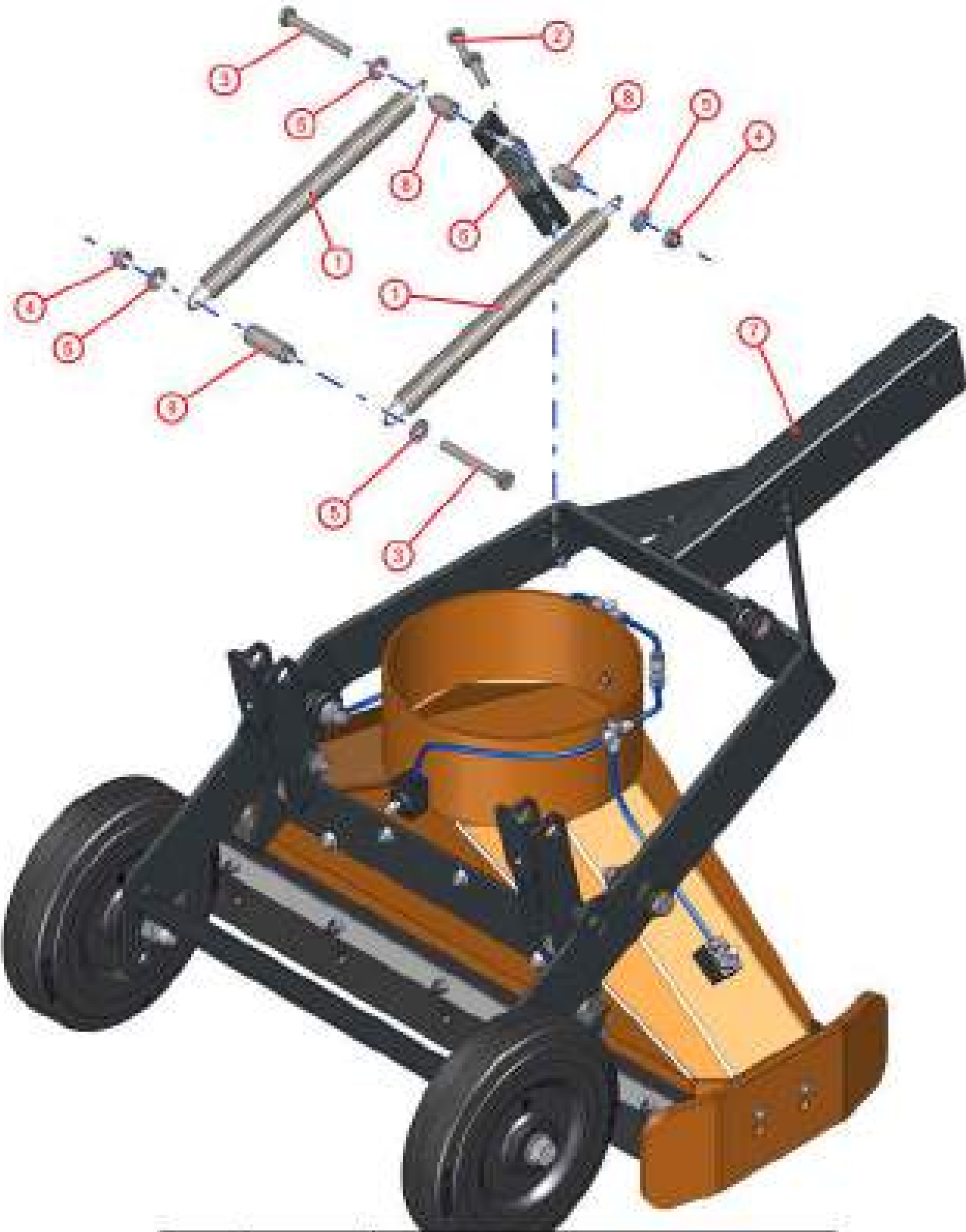
Suction nozzle - tilt return springs - right hand
