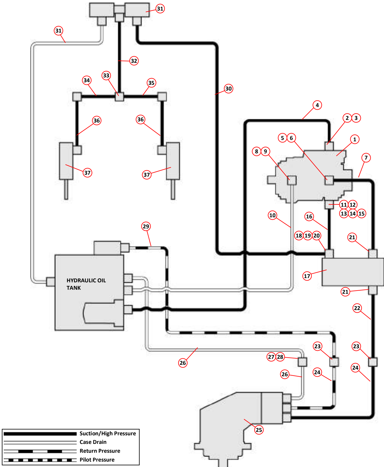
Hydraulic Circuit, Suction Fan and Variable Nozzle Tilt
