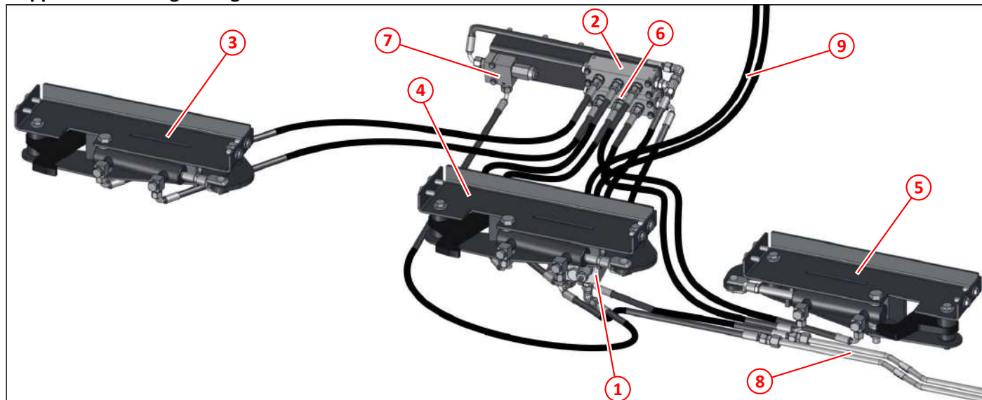
Figure 257: Hopper door locking arrangement
