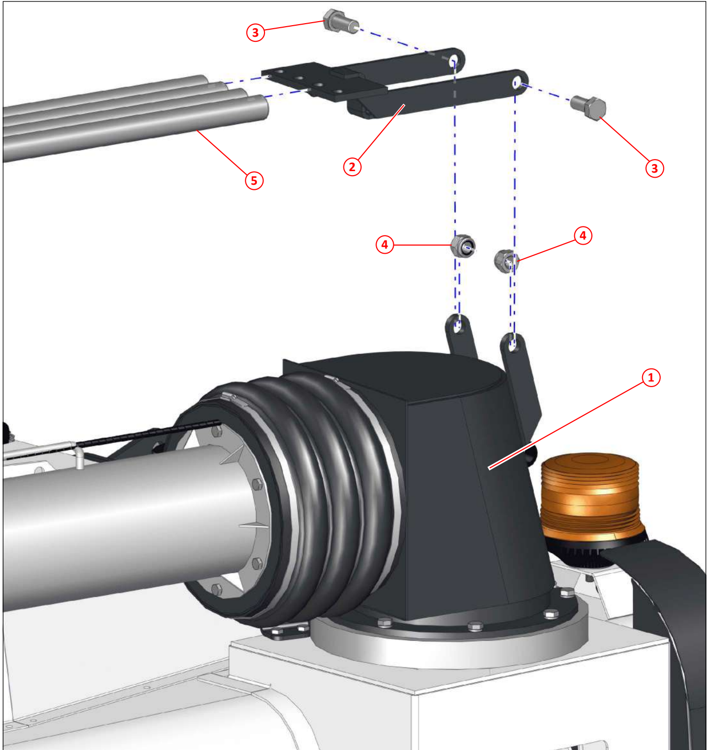
Figure 121: Overhead boom, spring anchor
