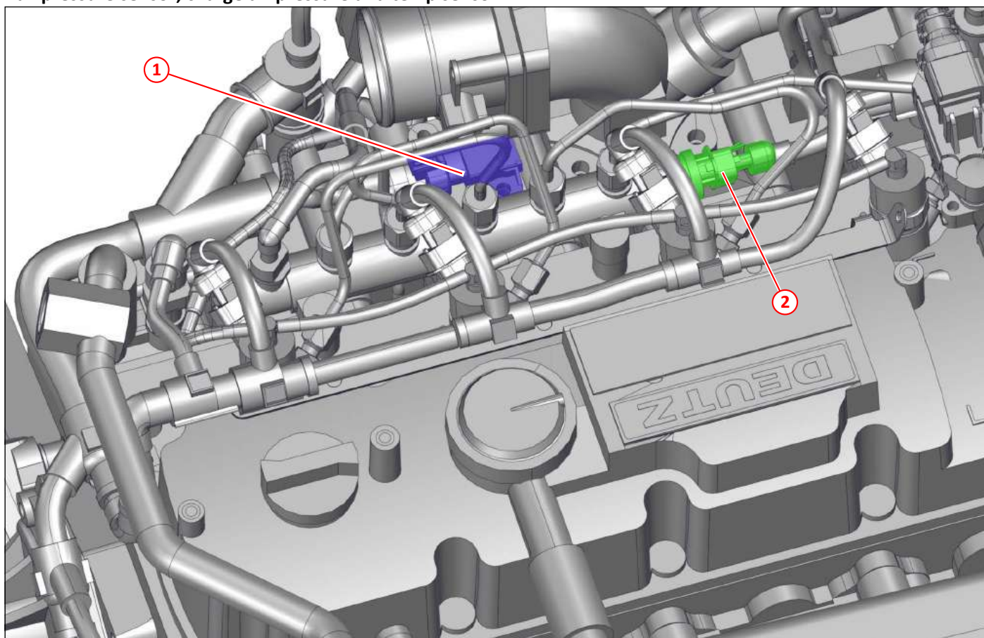
Figure 369: Rail pressure sensor, charge air pressure and temp sensor
