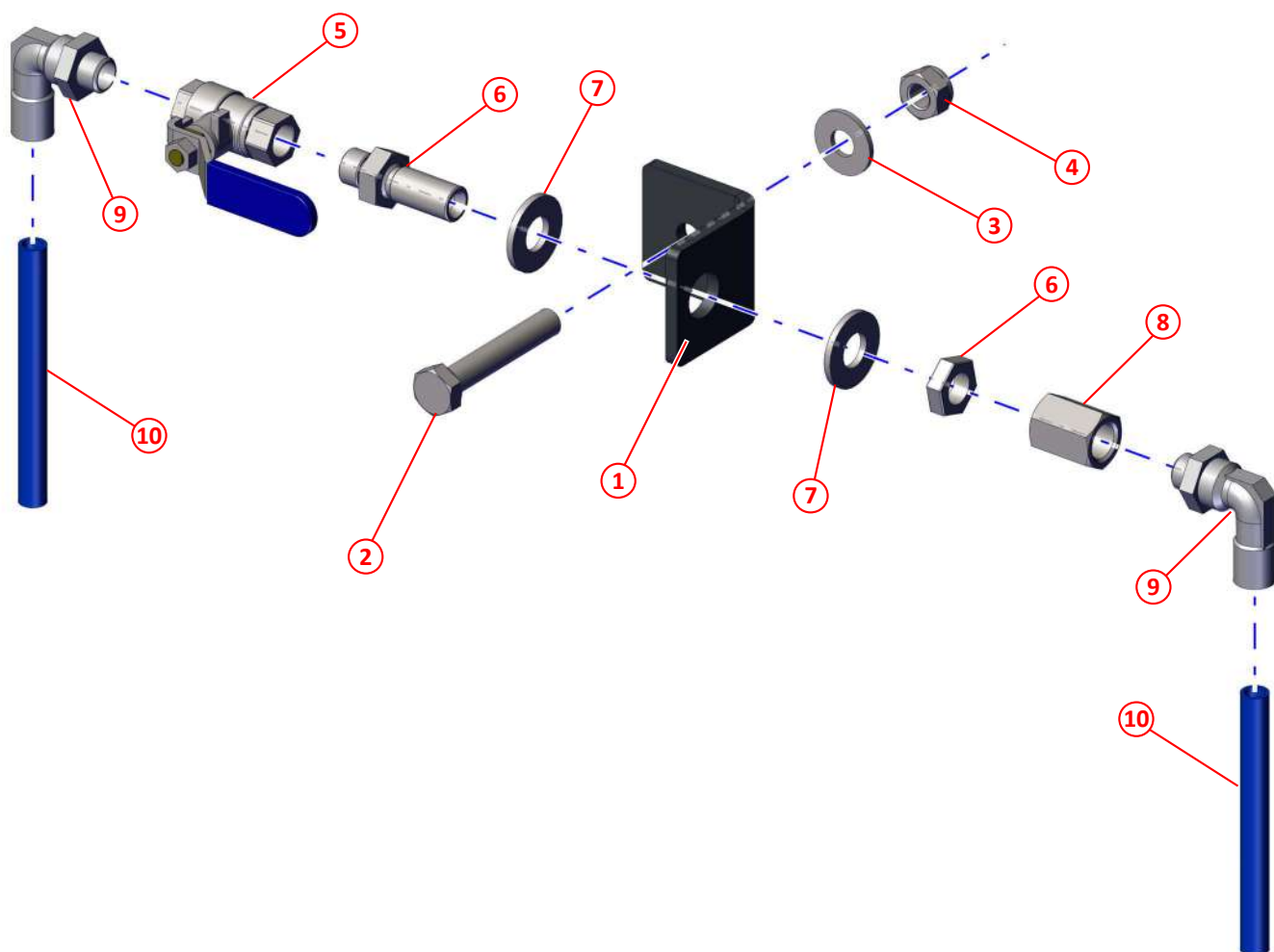
Figure 87: Manual water valve assembly, push fit, left hand - MYC
