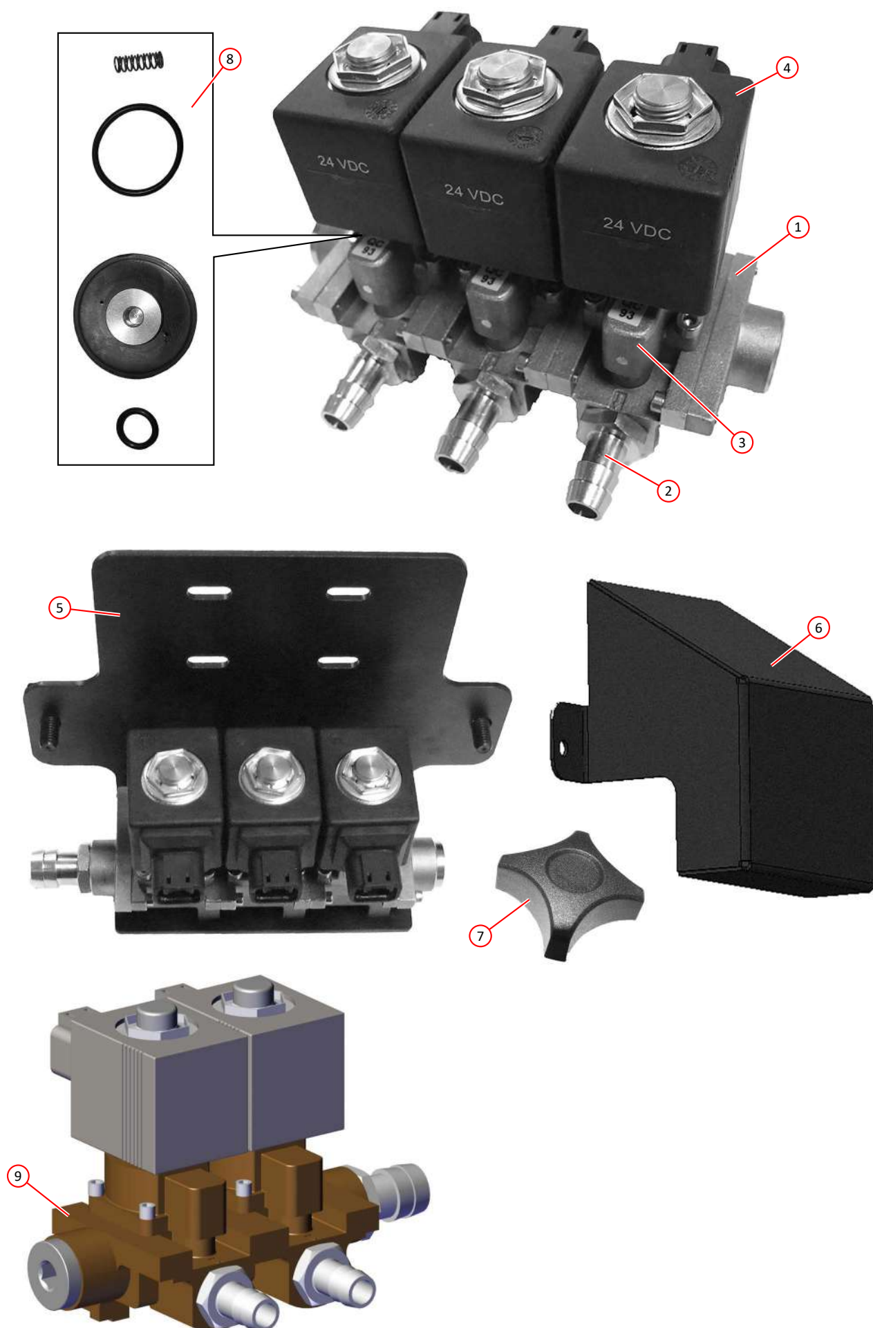
WATER VALVE ASSEMBLY
