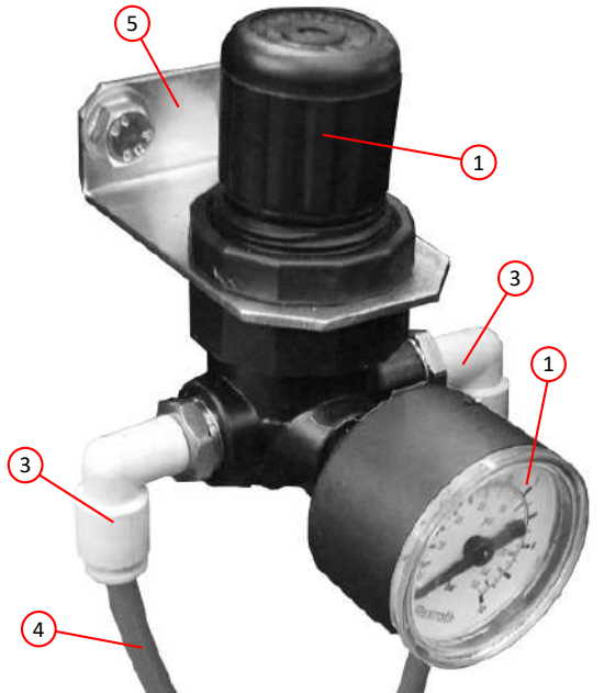
PRESSURE REGULATOR VALVE AND GAUGE
