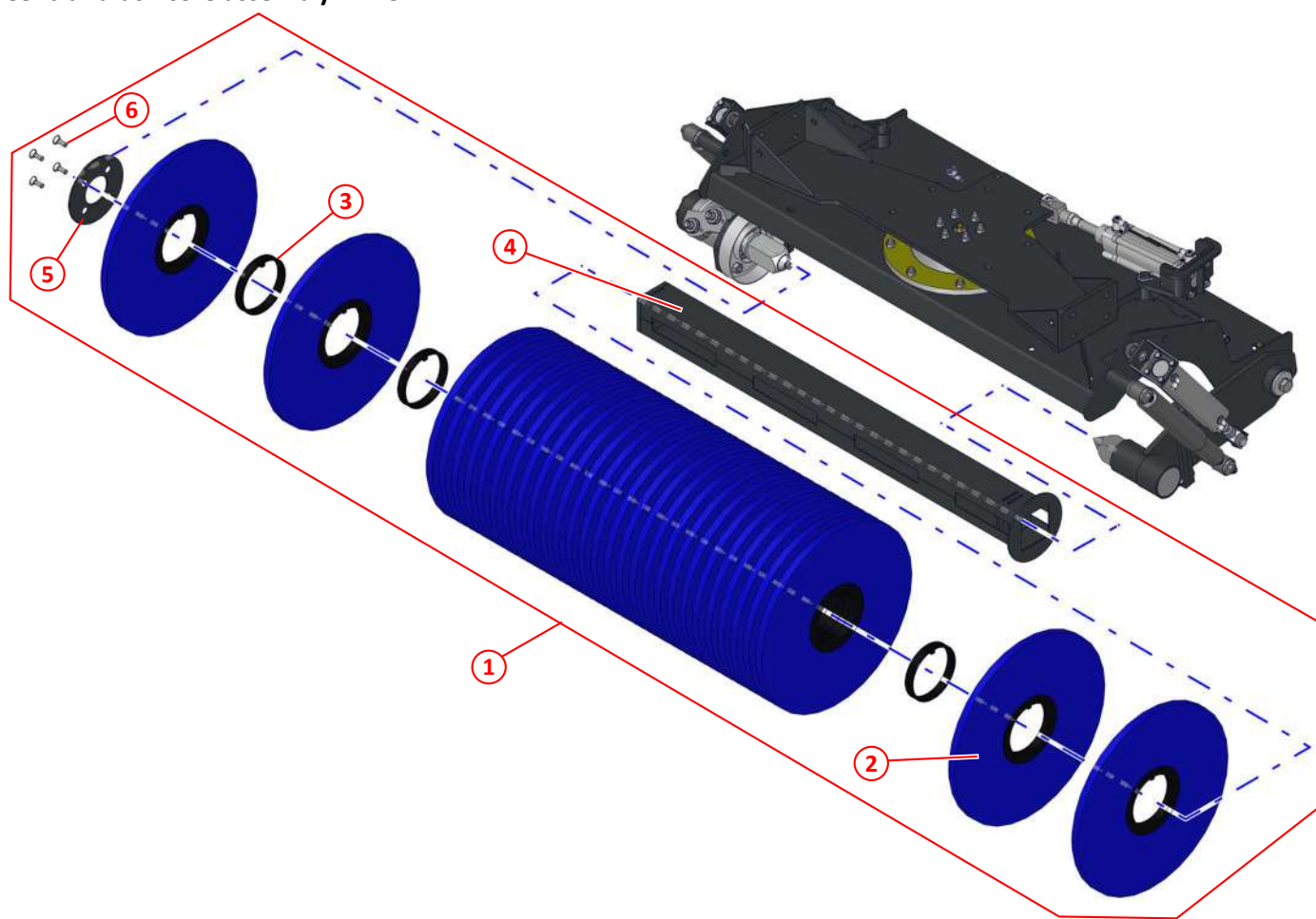
Figure 33: Central brush core assembly - MYC
