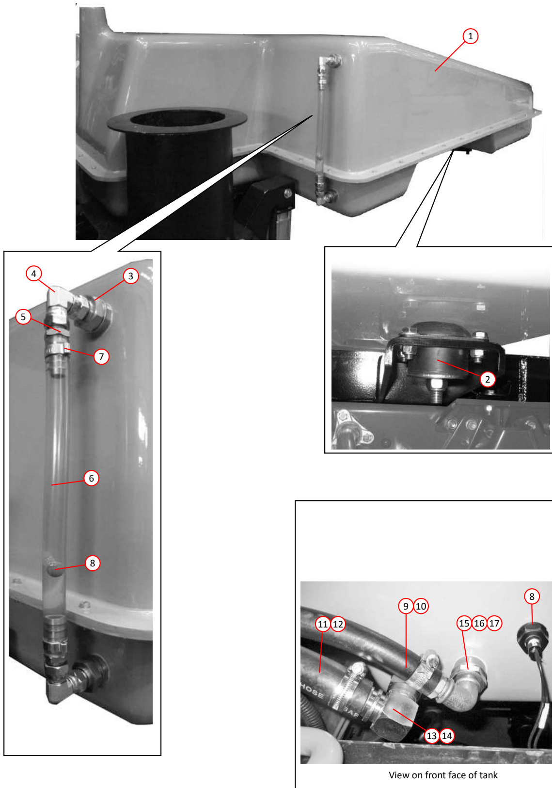
WATER TANK ASSEMBLY
