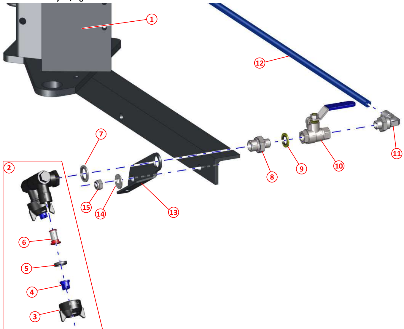
Figure 90: Side brush water jets, right hand - MYC
