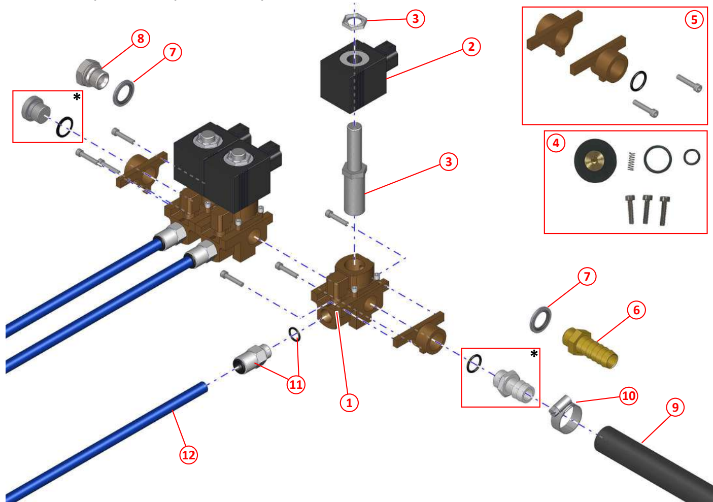
Figure 83: Water valves, push fit, low pressure, components - MYC
