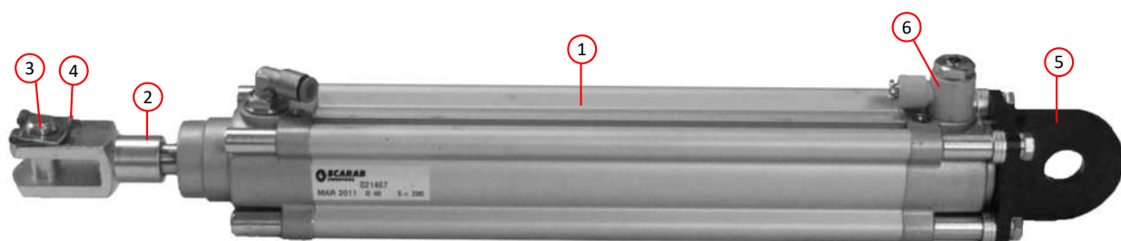
PNEUMATIC CYLINDER, AUTO BLANKING - ASSEMBLY
