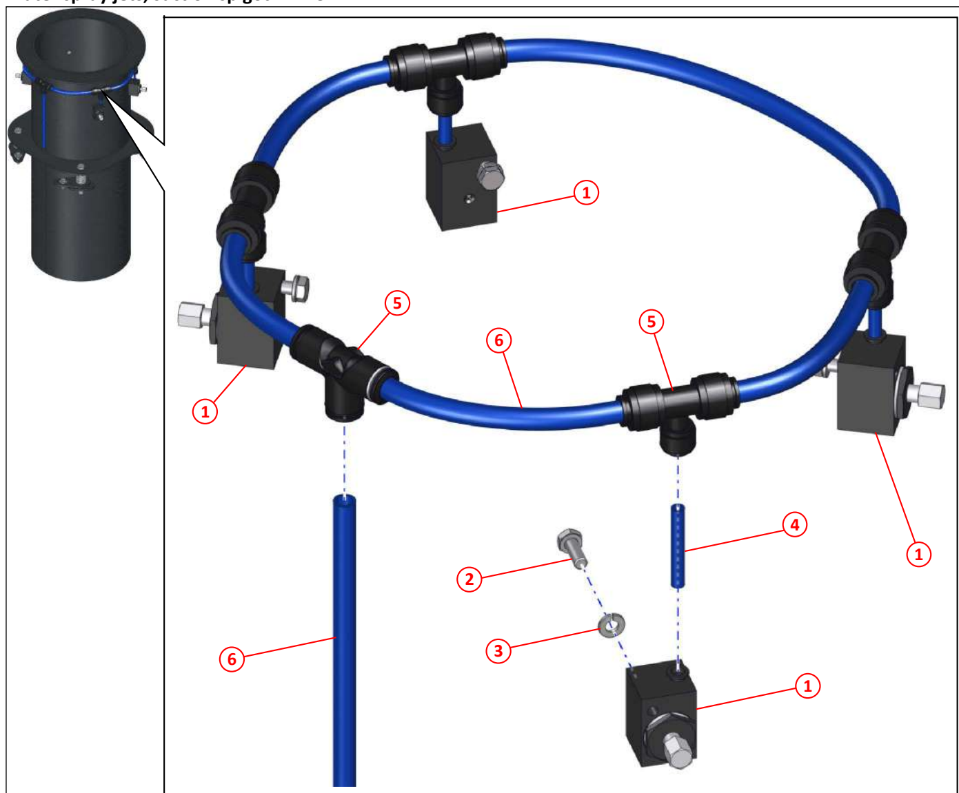
Figure 85: Water spray jets, suction spigot - MYC
