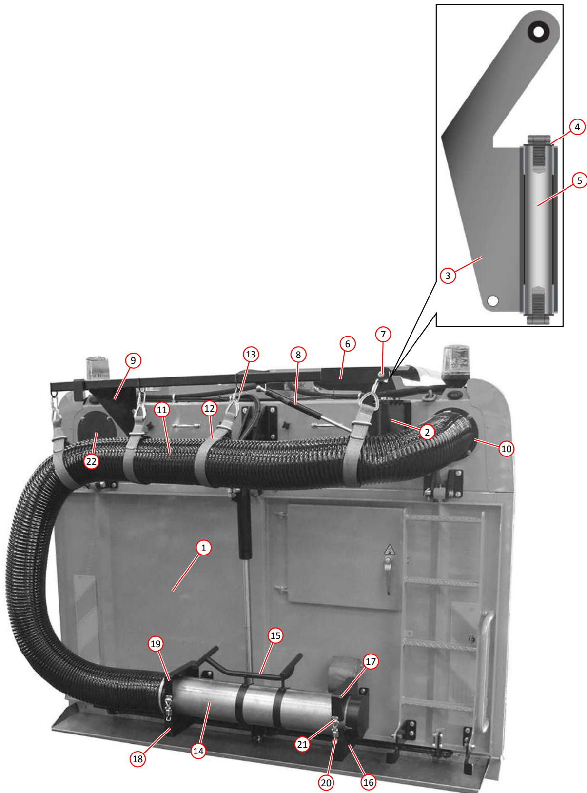
REAR WANDER BOOM ARRANGEMENT
