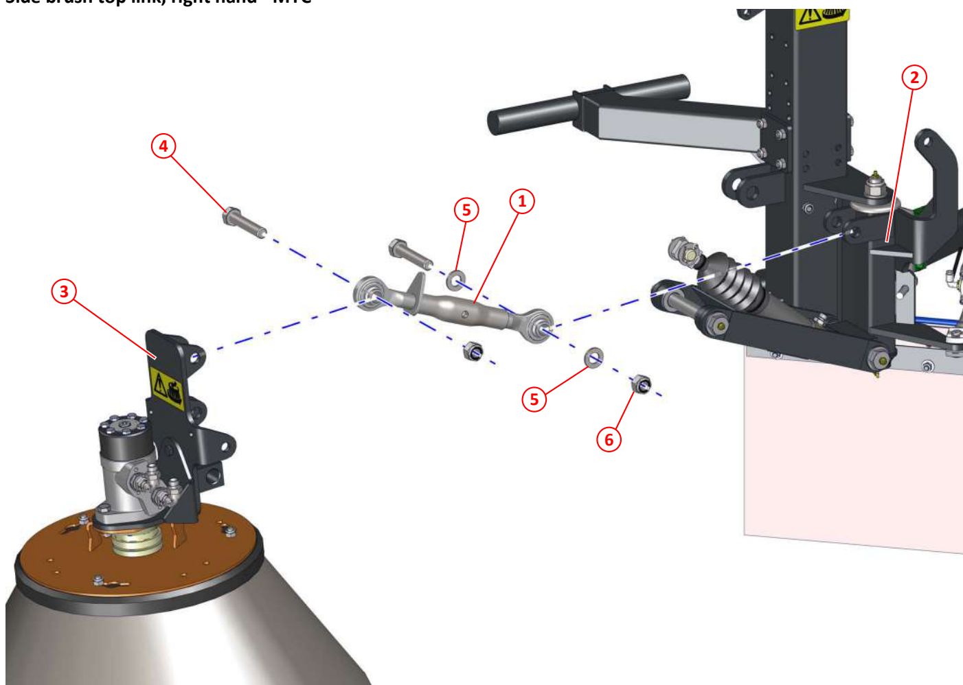
Figure 19: Side brush top link, right hand - MYC
