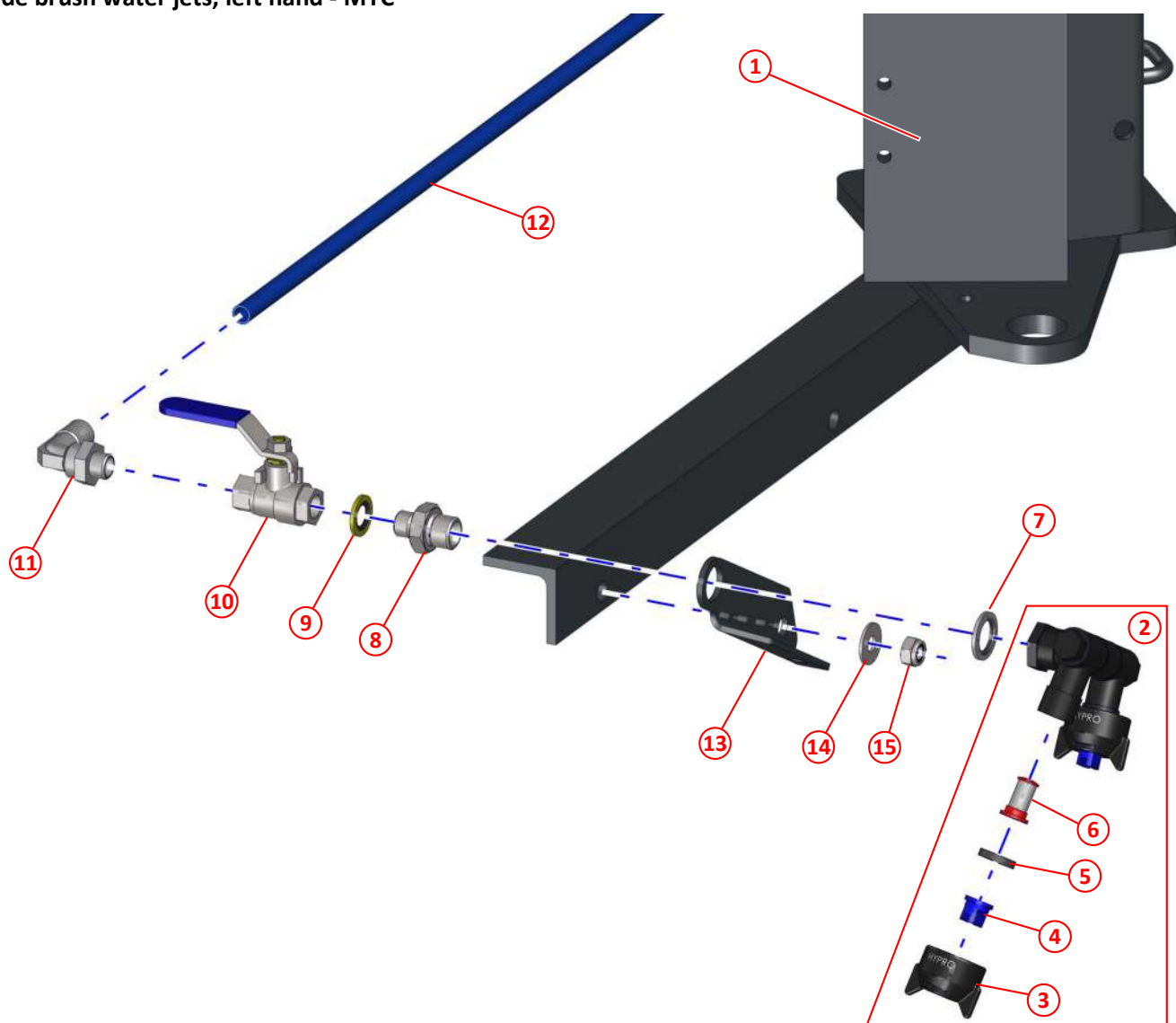
Figure 13: Side brush water jets, left hand - MYC
