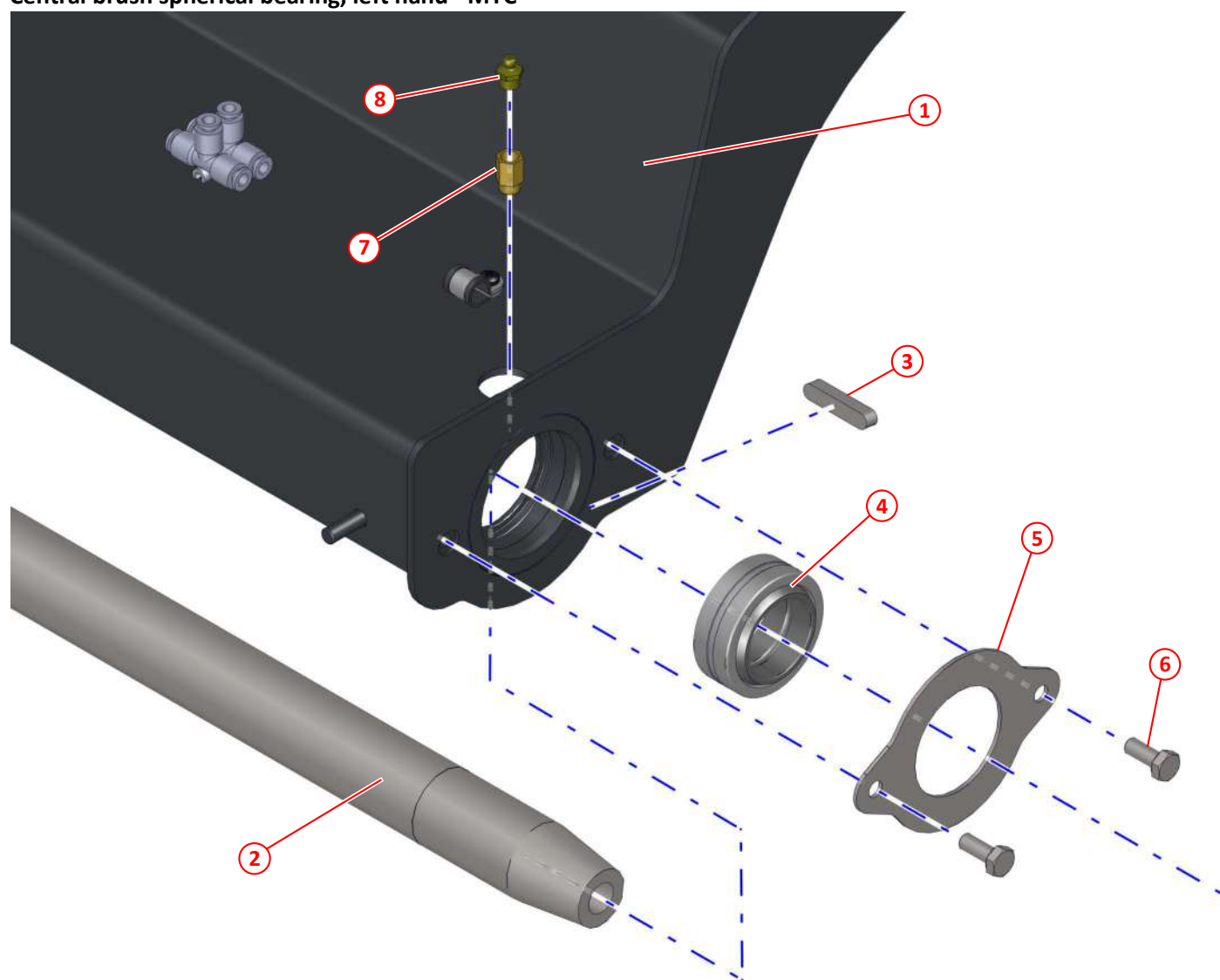
Figure 45: Central brush spherical bearing, left hand - MYC
