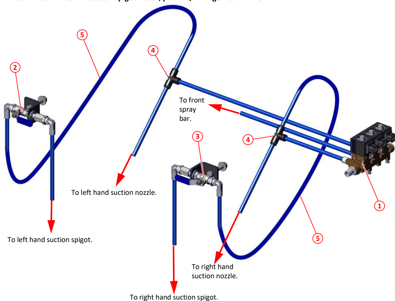
Figure 86: Manual water valves for suction spigot water, push fit, arrangement - MYC
