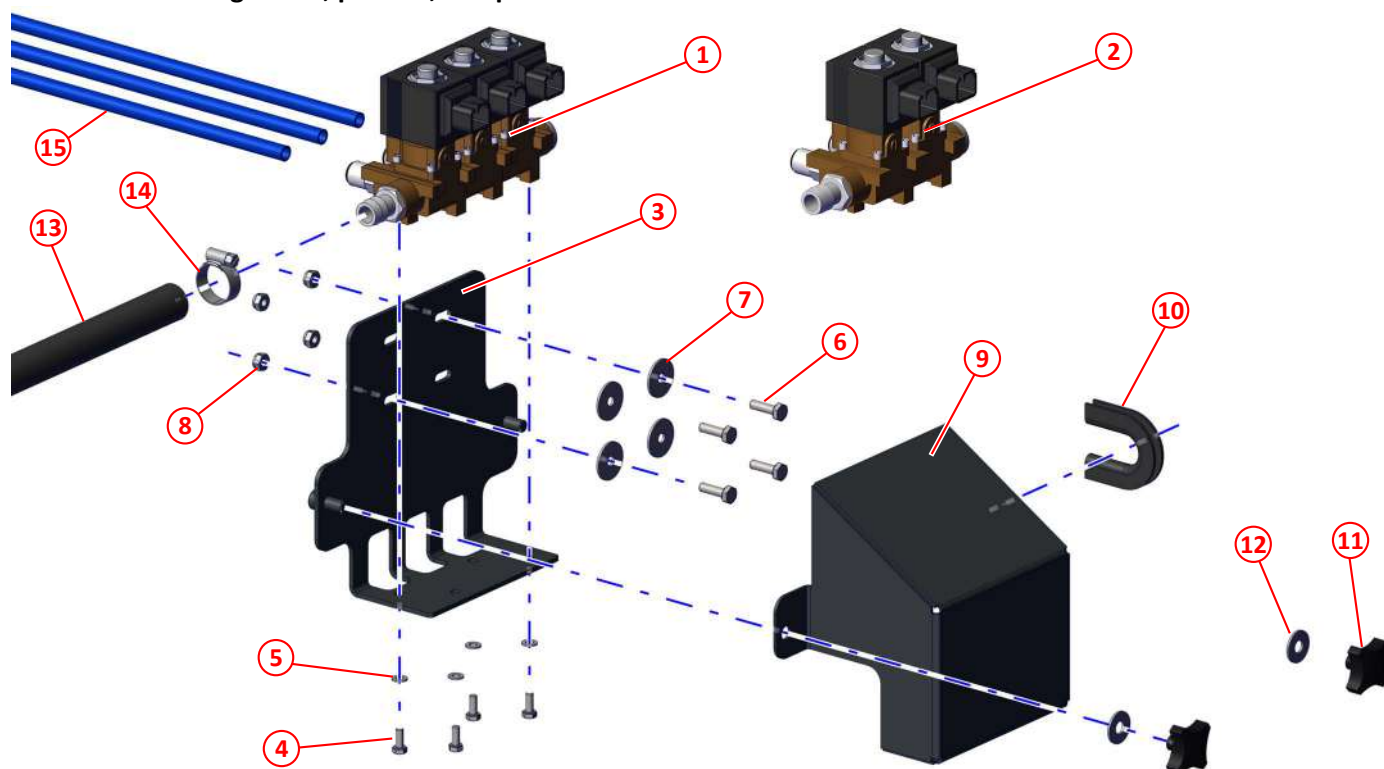
Figure 82: Water valve arrangement, push fit, low pressure - MYC
