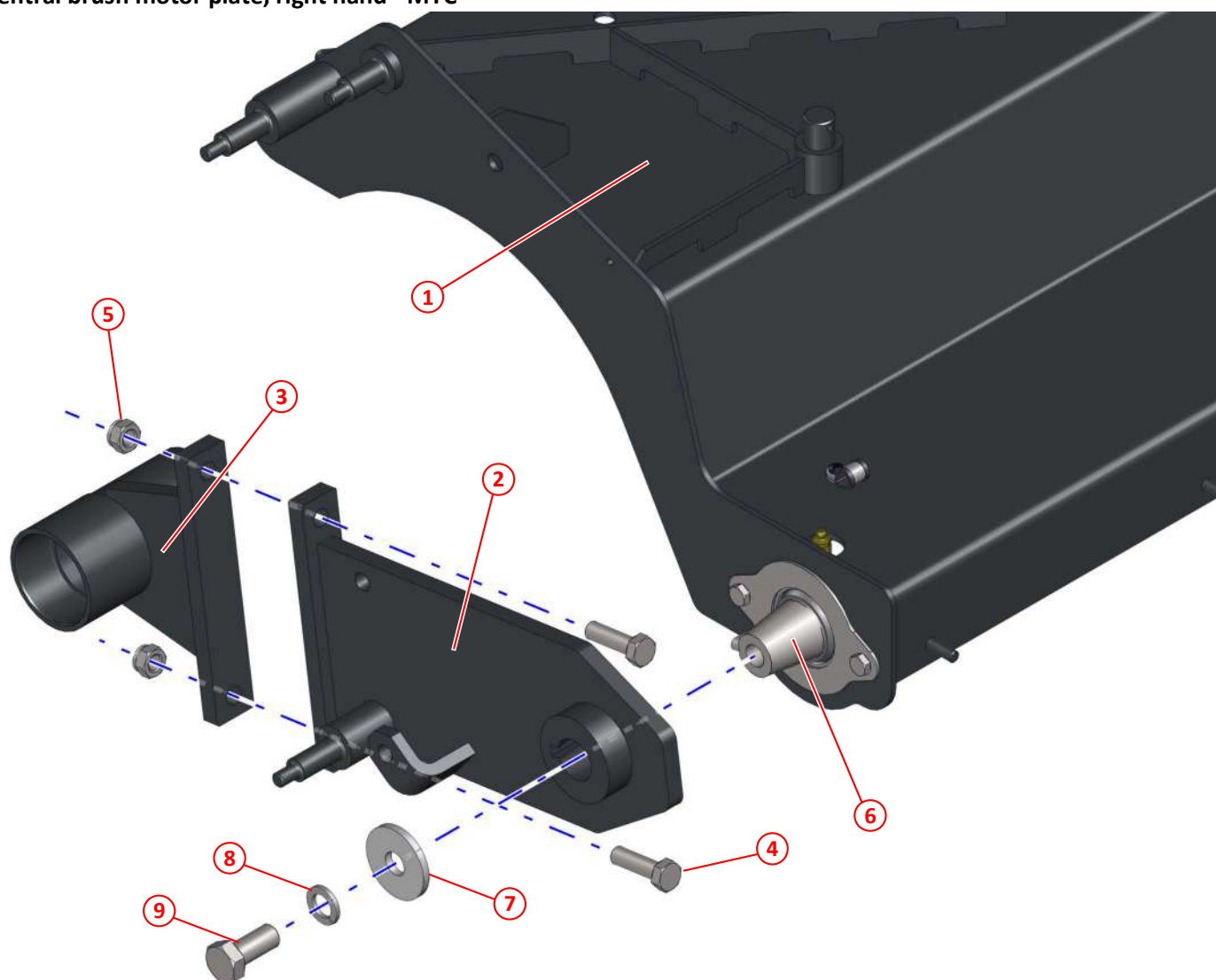
Figure 44: Central brush motor plate, right hand - MYC
