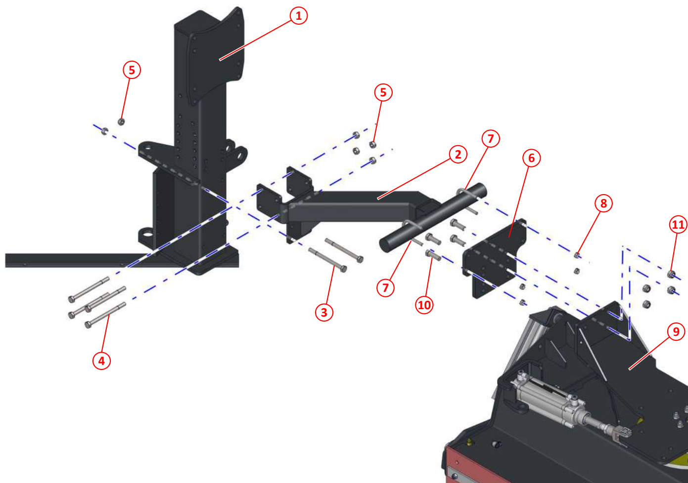
Figure 31: Central brush mounting, right hand - MYC
