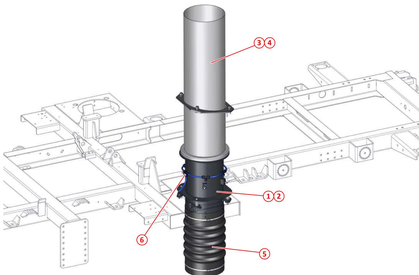
Figure 74: Suction spigot, deflector tube and suction hose arrangement - MYC
