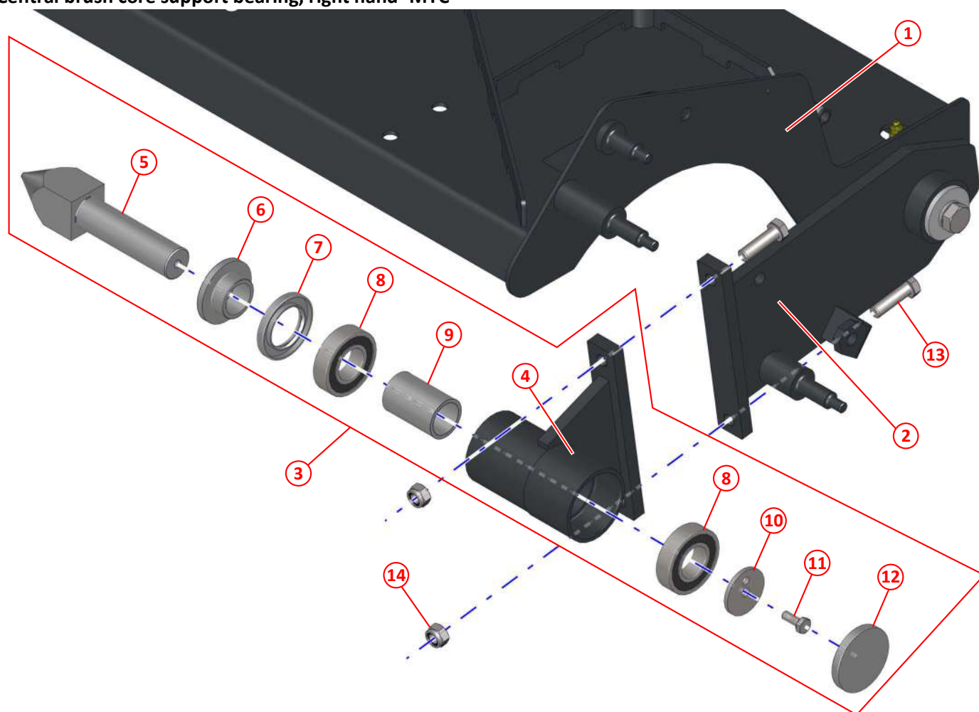
Figure 43: Central brush core support bearing, right hand- MYC
