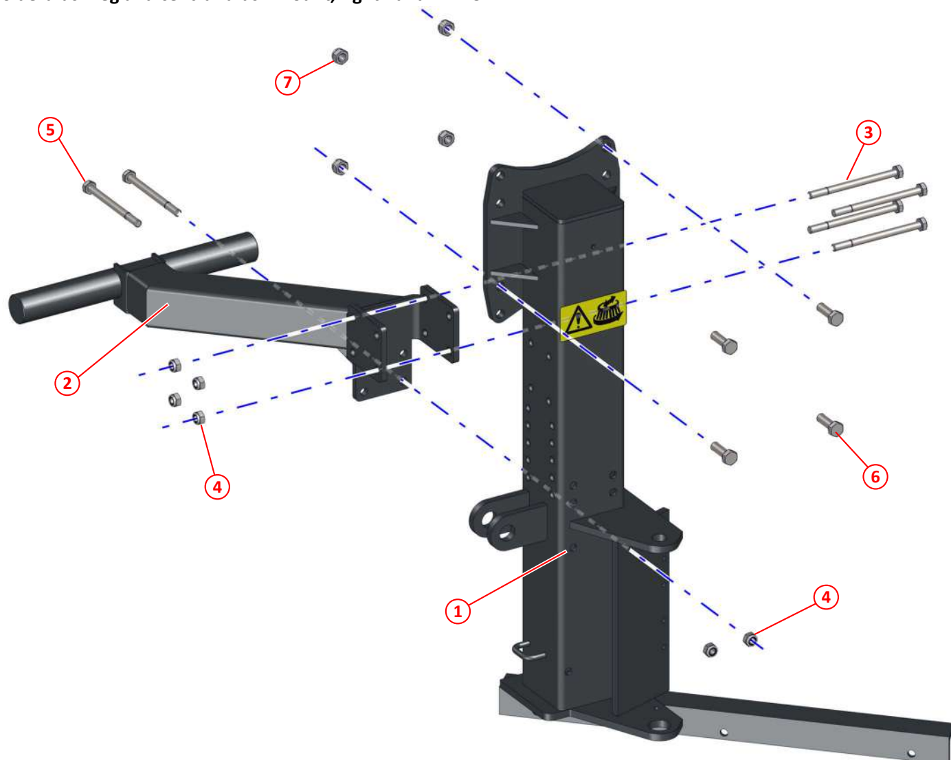
Figure 28: Side brush leg and central brush mount, right hand - MYC
