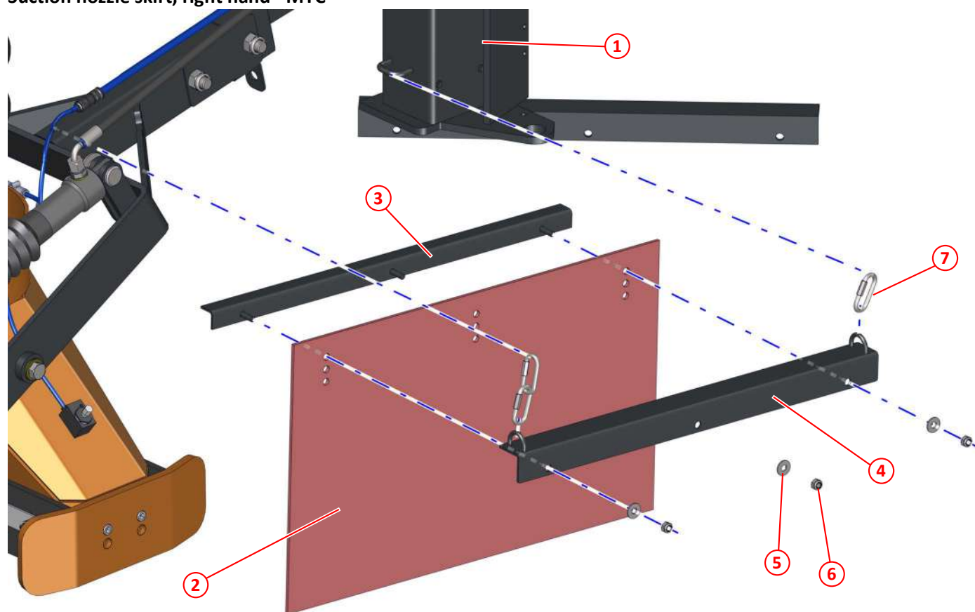
Figure 63: Suction nozzle skirt, right hand - MYC
