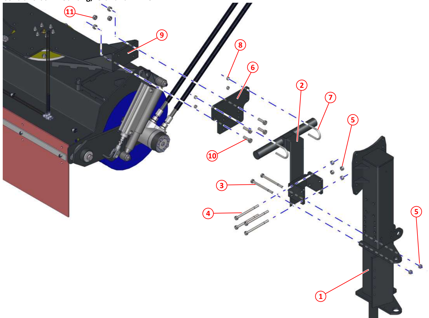
Figure 30: Central brush mounting, left hand - MYC
