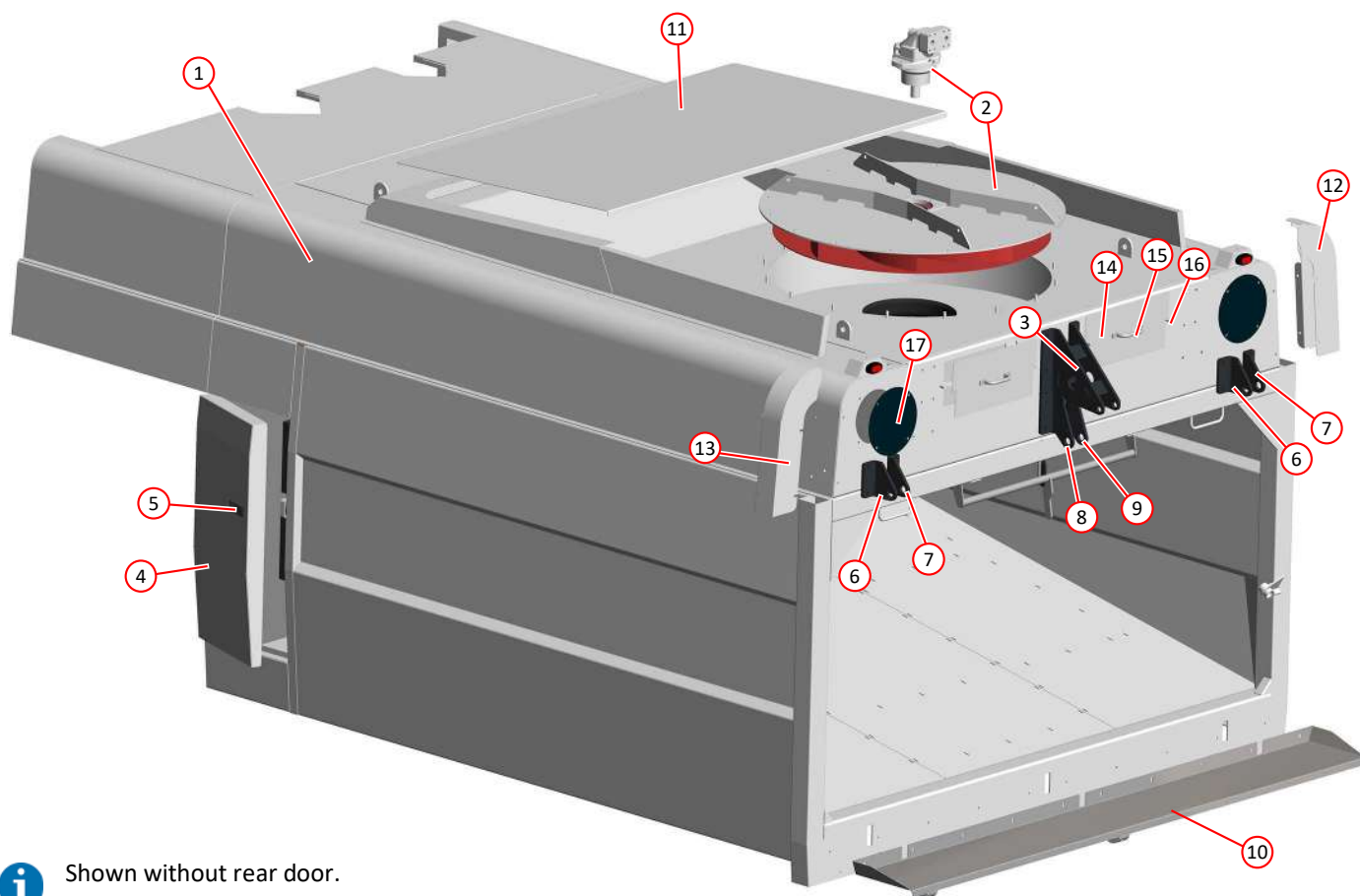
HOPPER GENERAL ARRANGEMENT
