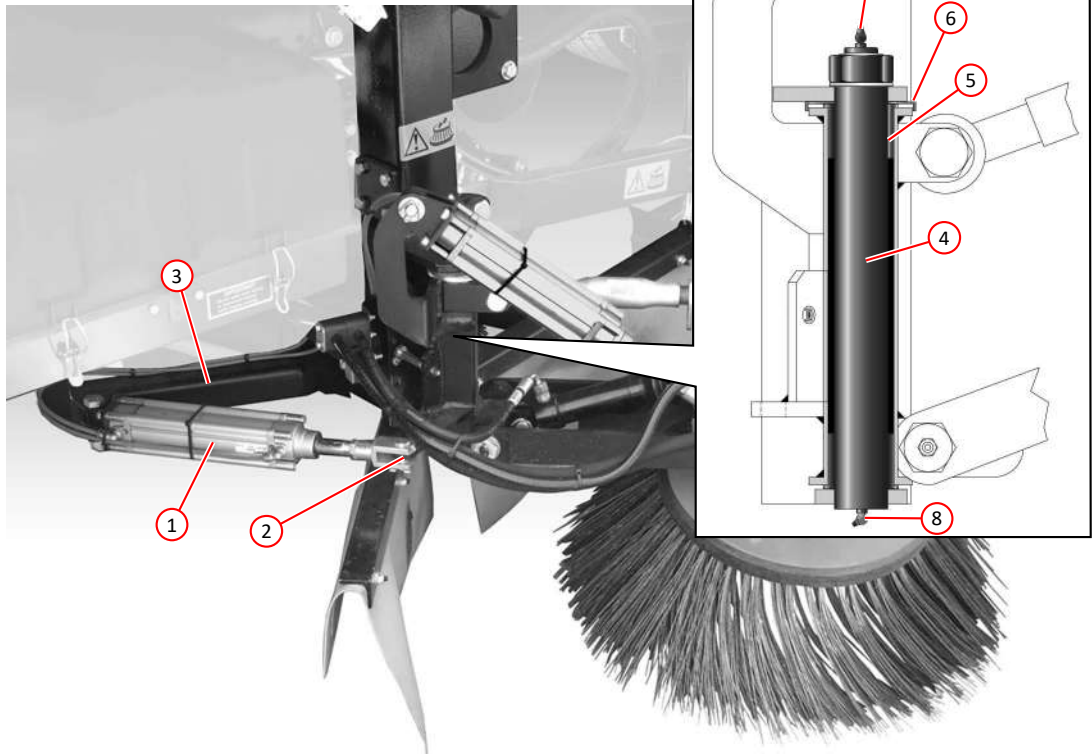
SIDE BRUSH SWING OUT ARRANGEMENT
