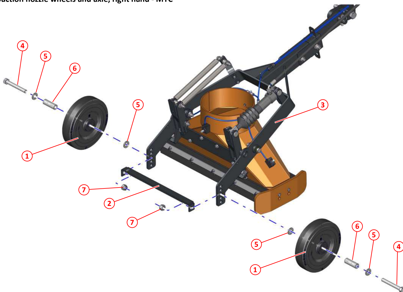
Figure 66: Suction nozzle wheels and axle, right hand - MYC
