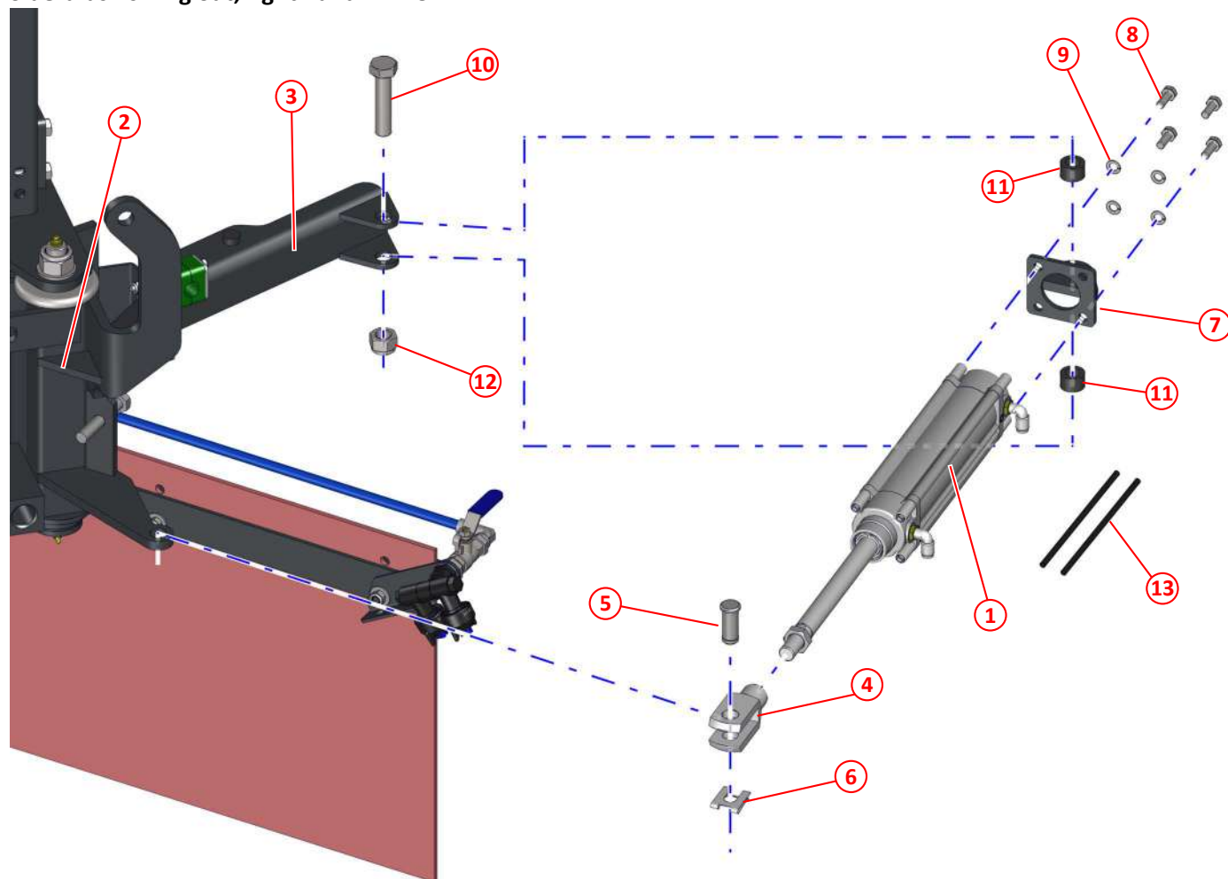
Figure 23: Side brush swing out, right hand - MYC
