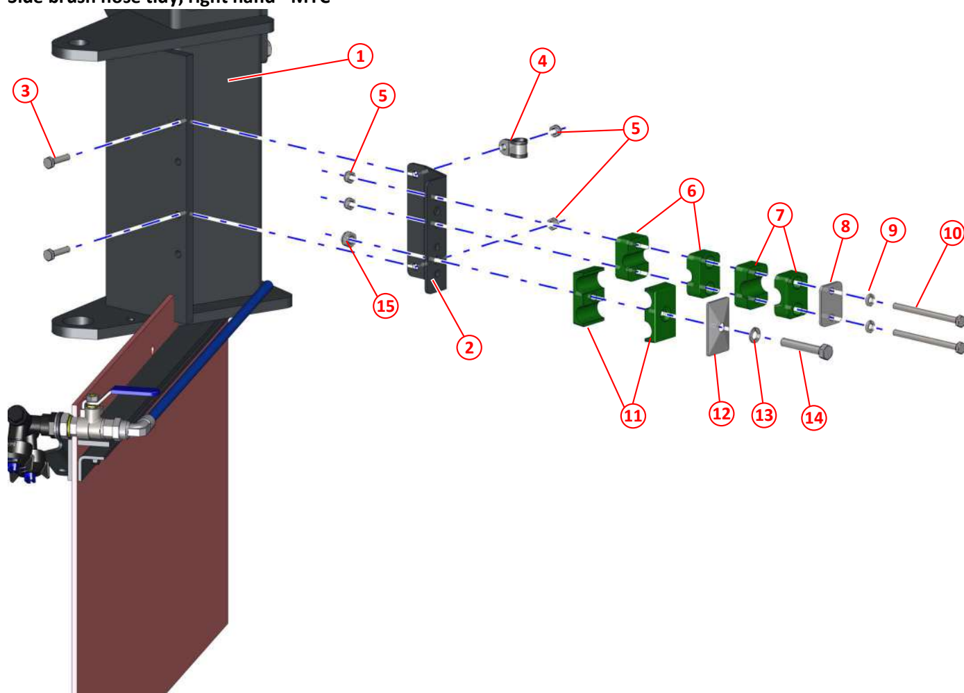
Figure 25: Side brush hose tidy, right hand - MYC
