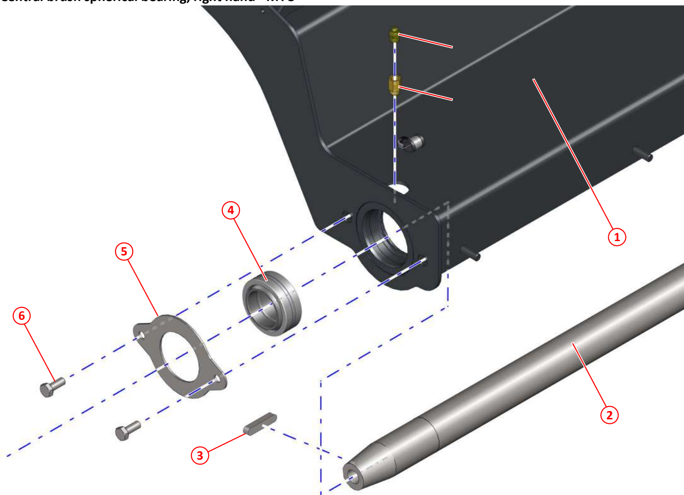
Figure 46: Central brush spherical bearing, right hand - MYC
