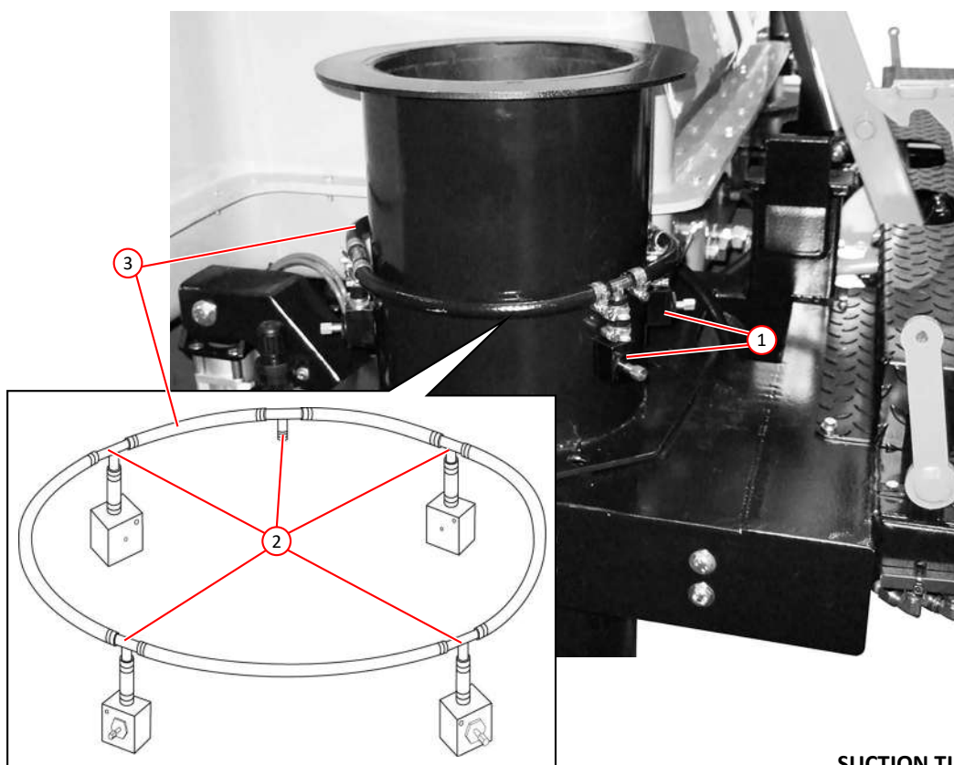
SUCTION TUBE DUST SUPPRESSION
