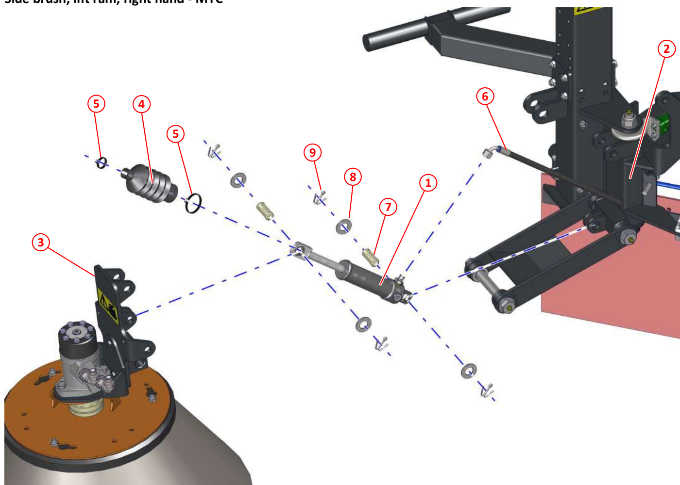
Figure 20: Side brush, lift ram, right hand - MYC
