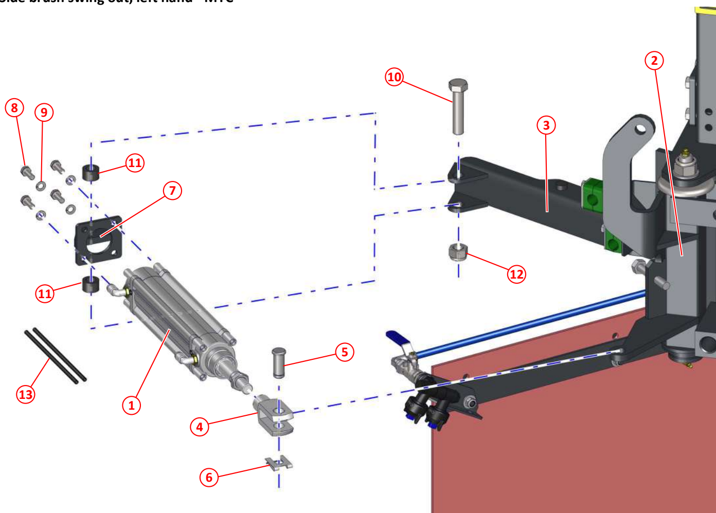
Figure 9: Side brush swing out, left hand - MYC
