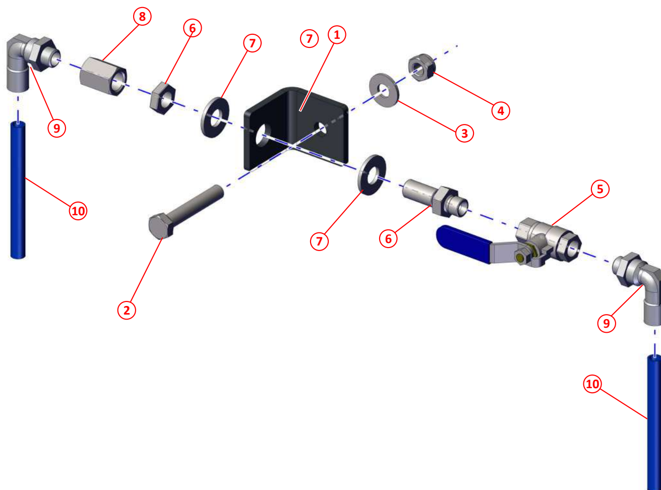
Figure 88: Manual water valve assembly, push fit, right hand - MYC
