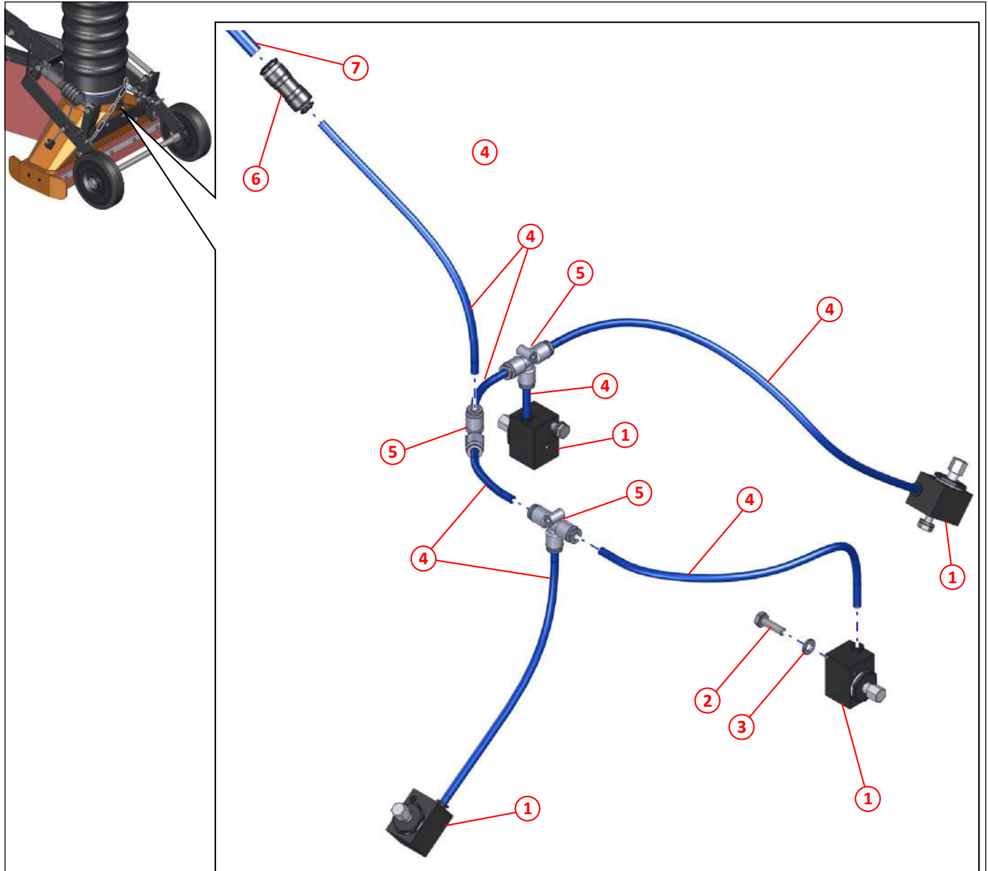
Figure 84: Water spray jets, suction nozzle - MYC
