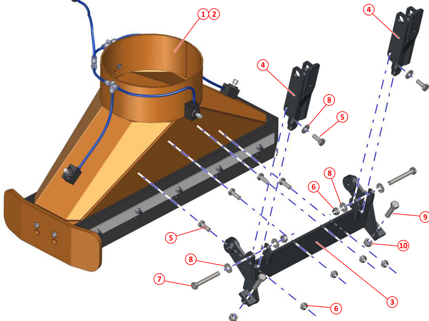
Figure 58: Suction nozzle pivot, left hand - MYC
