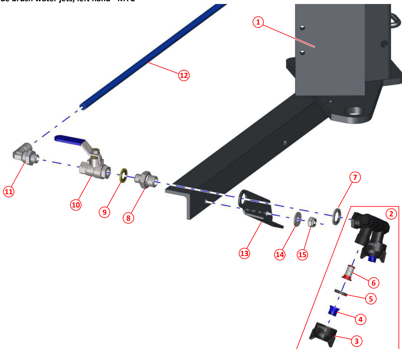
Figure 89: Side brush water jets, left hand - MYC
