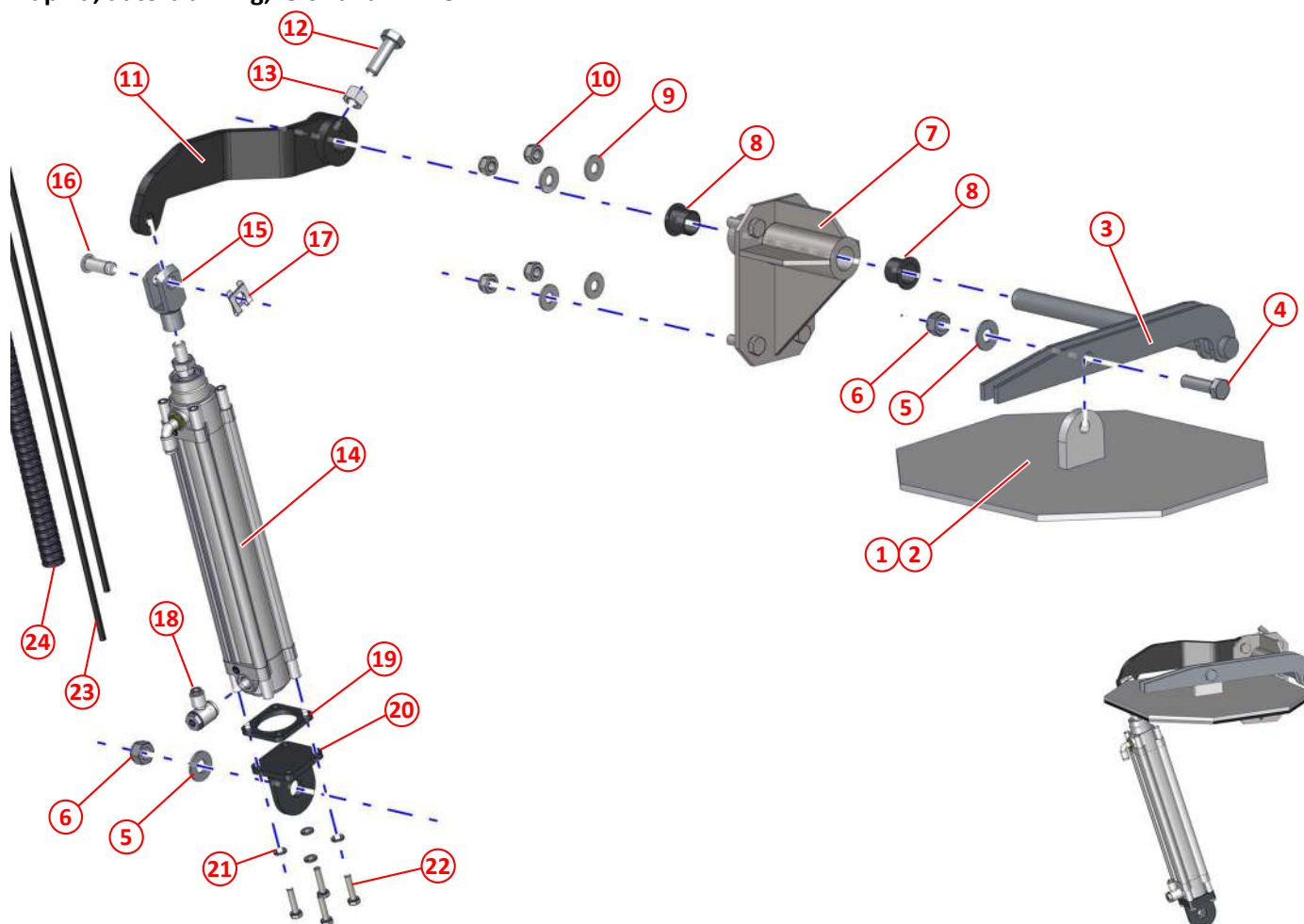
Figure 80: Flap lid, auto blanking - MYC
