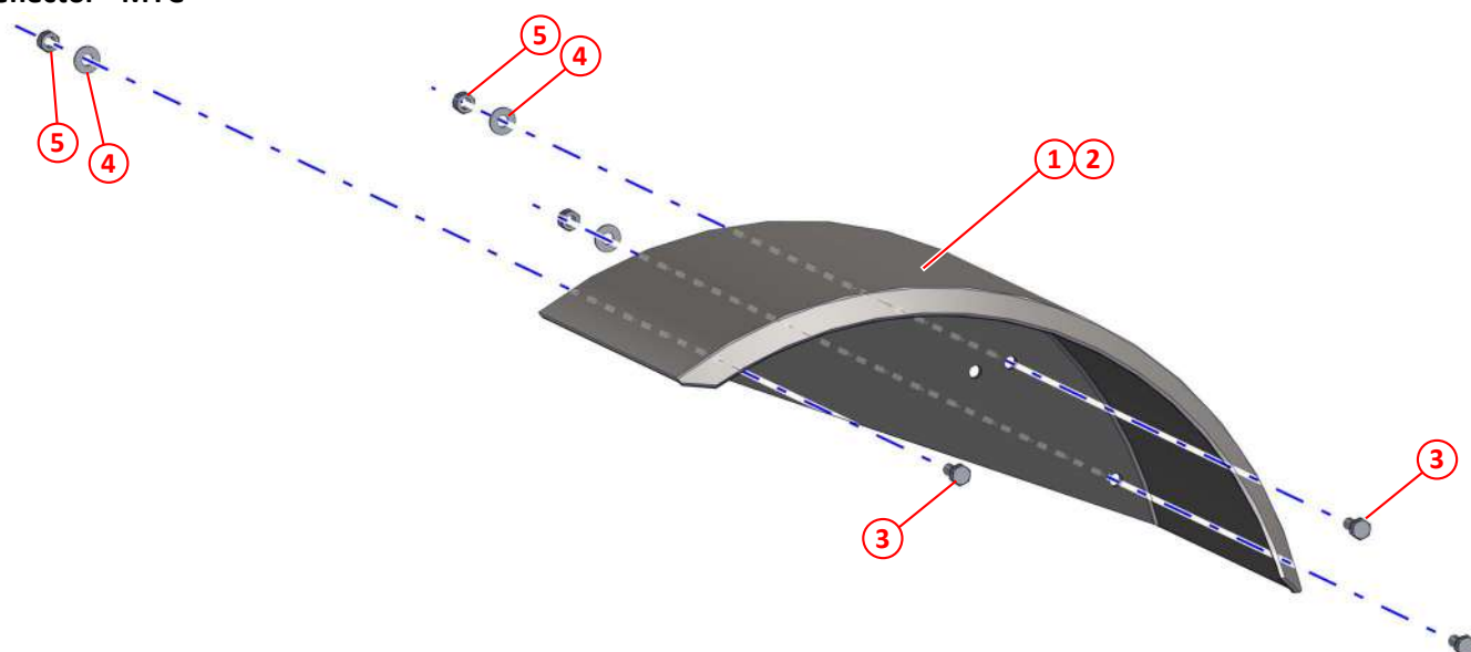
Figure 78: Deflector- MYC
