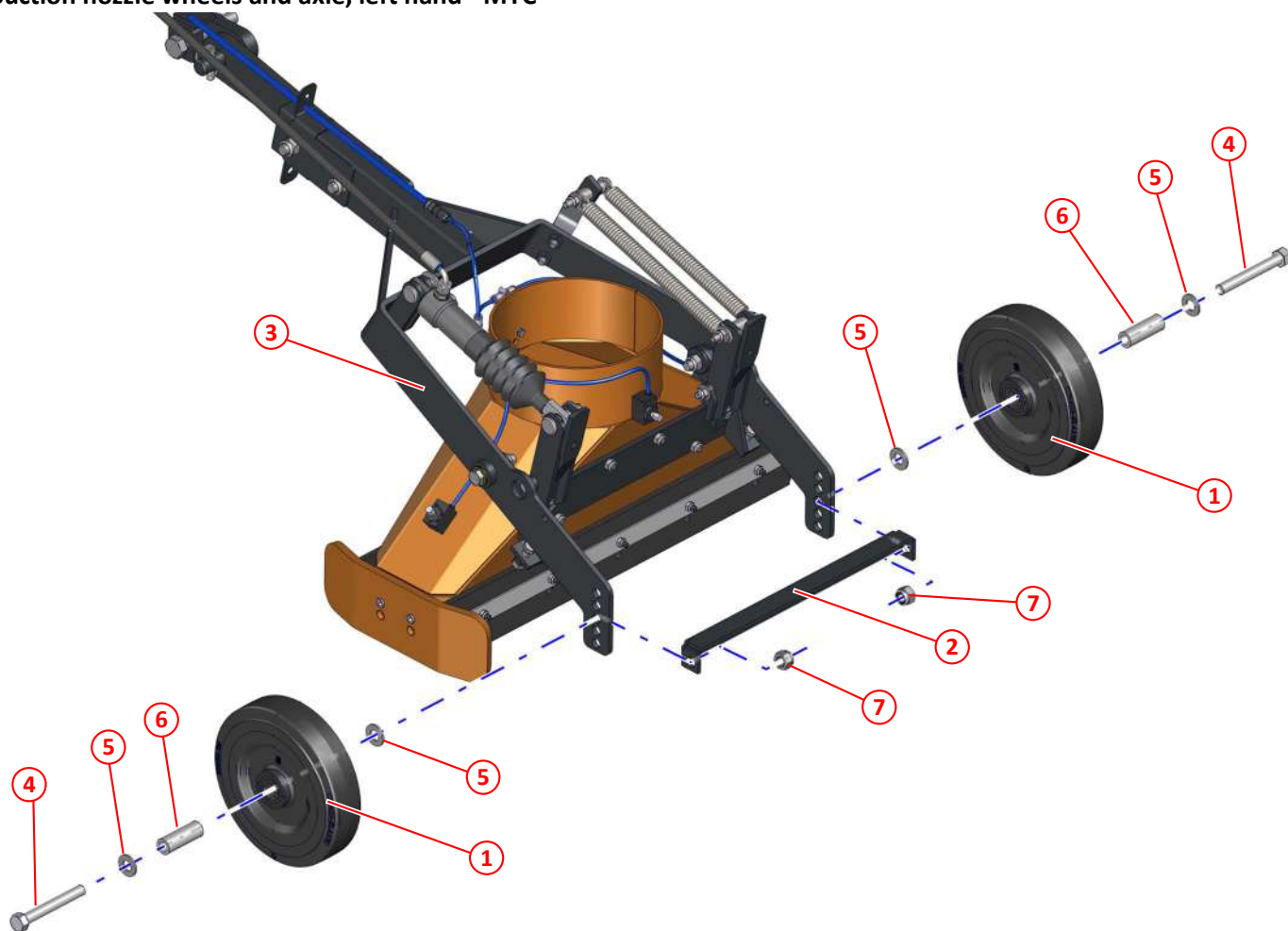
Figure 53: Suction nozzle wheels and axle, left hand - MYC
