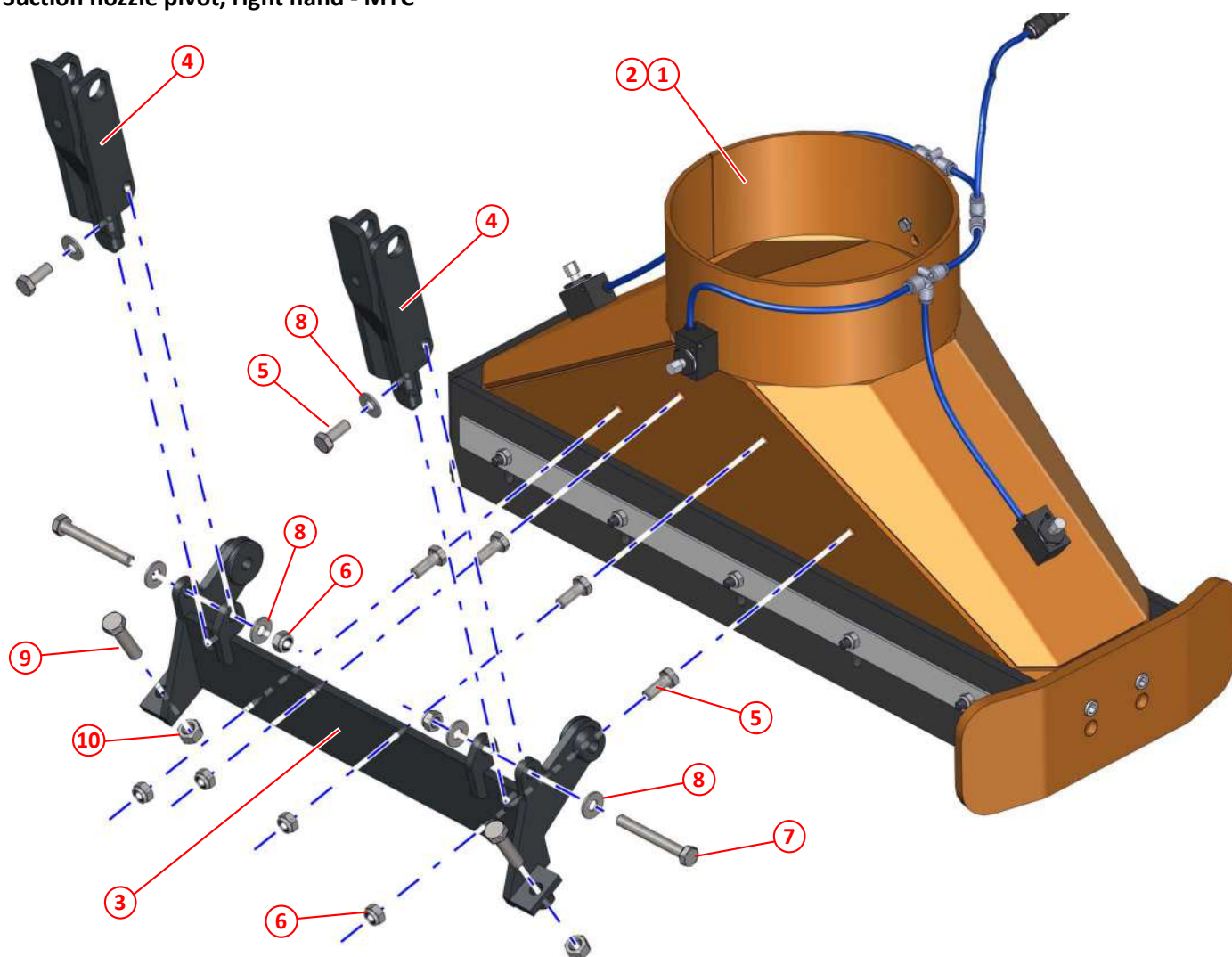
Figure 71: Suction nozzle pivot, right hand - MYC
