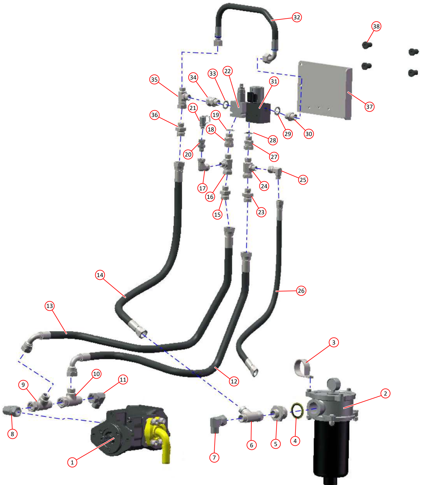
FAN CIRCUIT RELIEF AND DUMP VALVES
